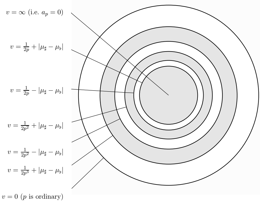
FIGURE 1. The locus inside the p -adic unit disc in which the modesty algorithm chooses \sharp or \flat when \frac{p-1}{4p^4} < |\mu_\sharp - \mu_\flat| < \frac{p-1}{4p^3} . Here, v = \text{ord}_p(a_p) indicates the possible valuations of a_p inside the unit disc. At the center, we have a_p = 0 , i.e. v = \infty . On the edge, we have v = 0 , so that p is ordinary. In the central shaded region, the formula involves \mu_\sharp, \lambda_\sharp for odd n and \mu_\flat, \lambda_\flat for even n , while in the second shaded region, \mu_\sharp and \lambda_\sharp are part of the formula for even n , and \mu_\flat and \lambda_\flat for odd n . In the outermost shaded region, the roles are flipped yet again and the \sharp -invariants come into play for odd n , and the \flat -invariants for even n . When \mu_\sharp < \mu_\flat , the formulas are only controlled by the \mu_\sharp and \lambda_\sharp in the non-shaded regions.
