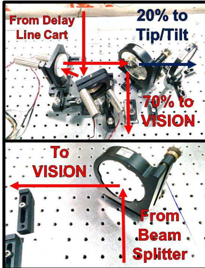
Fig. 3.— The light path towards the VISION beam combiner. (TOP) A minority (20%) of the light passes through the beam splitter in transmission to the tip/tilt mirrors for 1st order correction of the atmospheric turbulence. The majority (70%) of the light is reflected towards VISION. (BOTTOM) The light is re-routed towards the VISION beam combiner.
