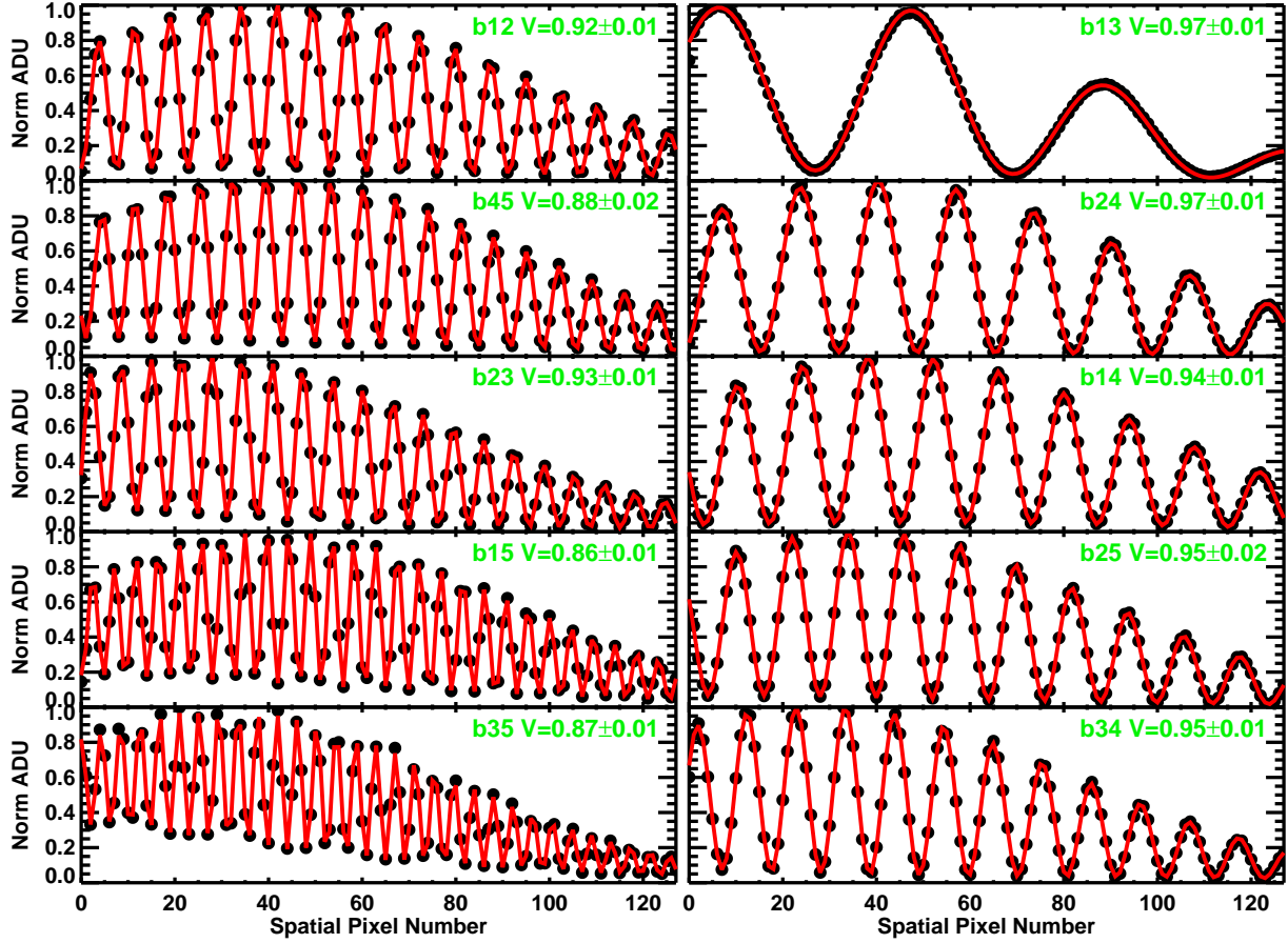
Fig. 8.— Interferograms using a 632.8 nm HeNe laser source and matched light paths for each beam pair for beams 1-5 (see §4.3). A fringe model was fit to each set of laser fringes for each beam pair using the fringe model Equation 8, and measure visibilities of 85-97%, which implies that the majority of light is interfering. The small visibility loss could be the result of polarization effects, beam intensity mismatch.
