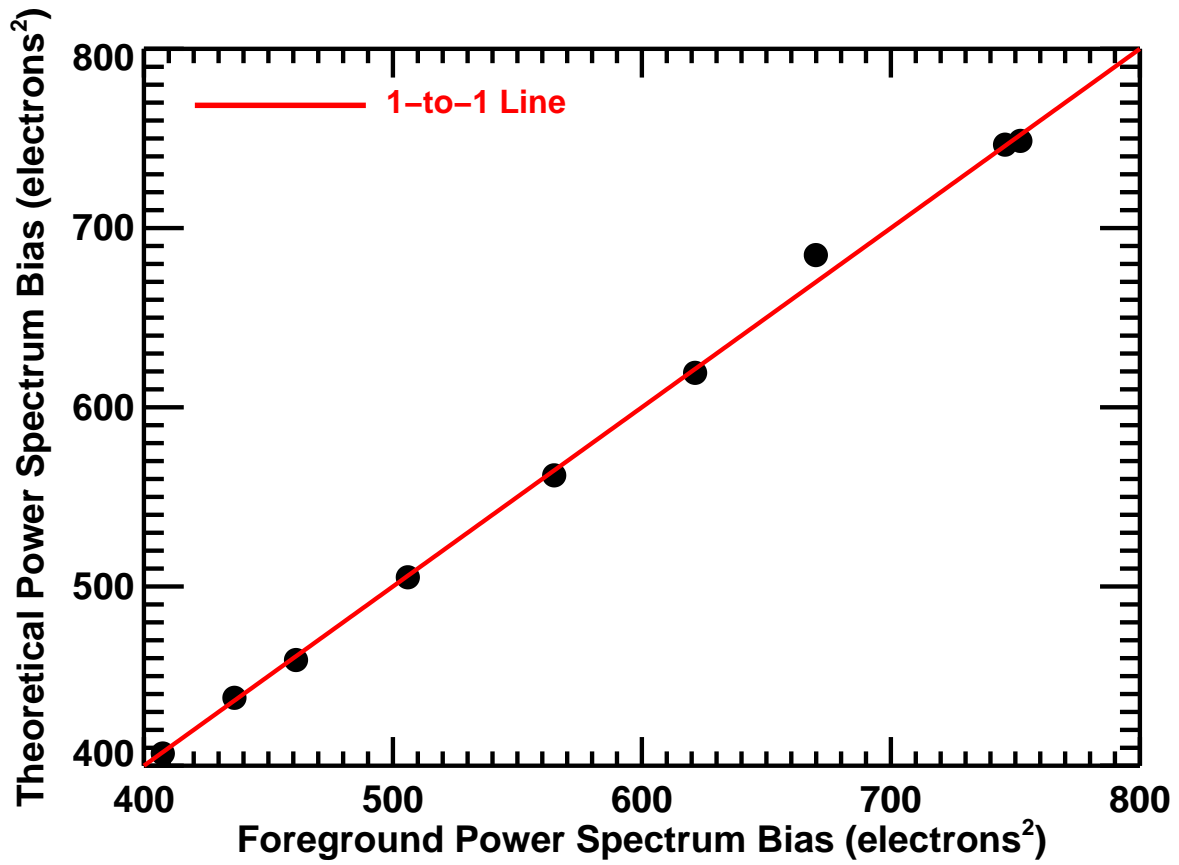
Fig. 15.— The theoretical power spectrum bias matches the foreground power spectrum for \gamma Orionis, further verifying that the bias correction procedures in the data-processing pipeline are accurate. The foreground amplitude of the bispectrum and power spectrum were averaged over 15.36 seconds, using 6 ms exposure times.
