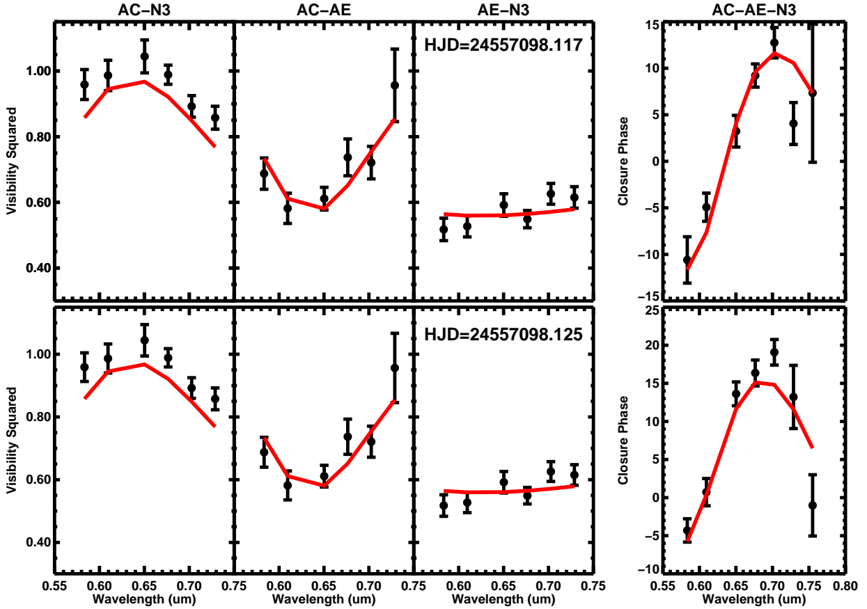
Fig. 16.— Sample calibrated squared visibilities and closure phase observations of \zeta Orionis on UT 03152016 at two different times of the night. The red solid line is the best fit model to the data. the best fit model for this binary star at the epoch the observations yields a separation of 40.6 \pm 1.8 mas, a position angle of 223.9 \pm 1.0^\circ for observations from 580 – 750 nm, in good agreement with the predicted separation of 40.1 \pm 1.0 mas and position angle 223.2 \pm 2.3 mas from Hummel et al. (2013). The observed flux ratio of 2.18 \pm 0.13 mag is also in good agreement with the flux ratio 2.2 \pm 0.1 mag from Hummel et al. (2013). The AC-N3 visibilities have a small bias likely due possibly to imperfect photometric calibration.
