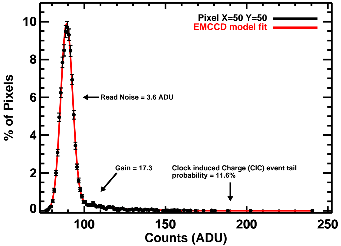
Fig. 12.— Sample fit to a histogram of a time series of \approx 10^5 dark frames for pixel (50, 50), (black circles). The gain, read noise, and clock induced charge rate are derived by fitting an analytic EMCCD model to the data (red line). The analytic EMCCD model (see §5.1) is the convolution of the probability that a pixel only has read noise, or has read noise and a clock induced charge event.
