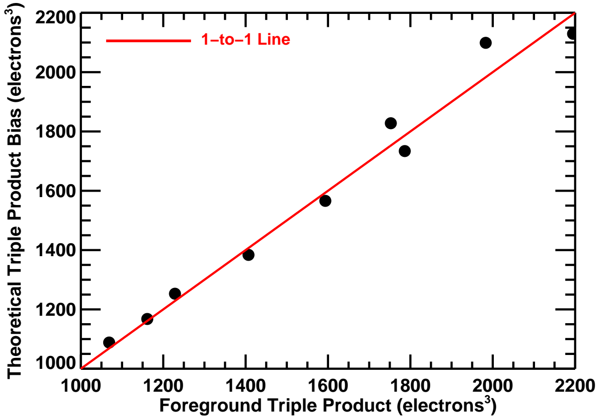
Fig. 14.— The theoretical bispectrum matches the amplitude of foreground bispectrum for \gamma Orionis, further verifying that the bias correction procedures in the data-processing pipeline are accurate. The foreground amplitude of the bispectrum and power spectrum were averaged over 15.36 seconds, using 6 ms exposure times.
