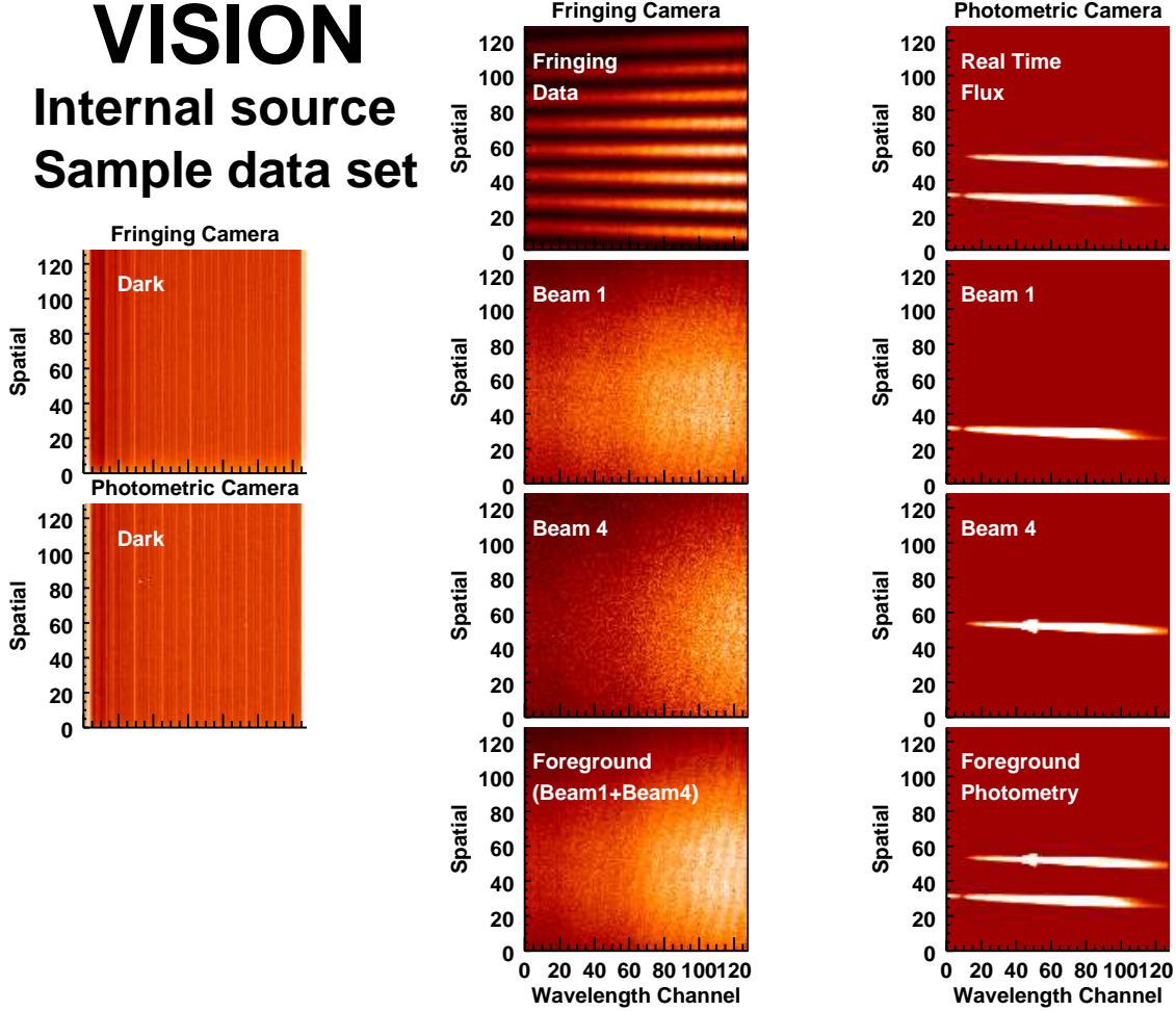
Fig. 5.— Sample VISION data set using an laboratory white light source with an R = 1000 spectrograph. A complete VISION data set to measure visibilities and closure phases includes (1) an average dark frame for both the fringing and photometric cameras to characterize the bias count structure across the EMCCDs, (2) the fringing data and simultaneous real-time flux measurements, (3) frames with light from each beam individually on the fringing and photometric cameras to measure the split of the light from the polarizing beam splitter, and (4) the foreground data to characterize the bias in the power spectrum (visibility bias) and the bispectrum. The small fringing seen in the foreground data is due to pixel-to-pixel sensitivity of the EMCCD chips. This pixel-to-pixel sensitivity only appears strongly after averaging at least 10 minutes of frames. The small point sources of light on the photometric camera frames are due to leakage of the laser metrology used by the delay line carts onto the EMCCDs.
