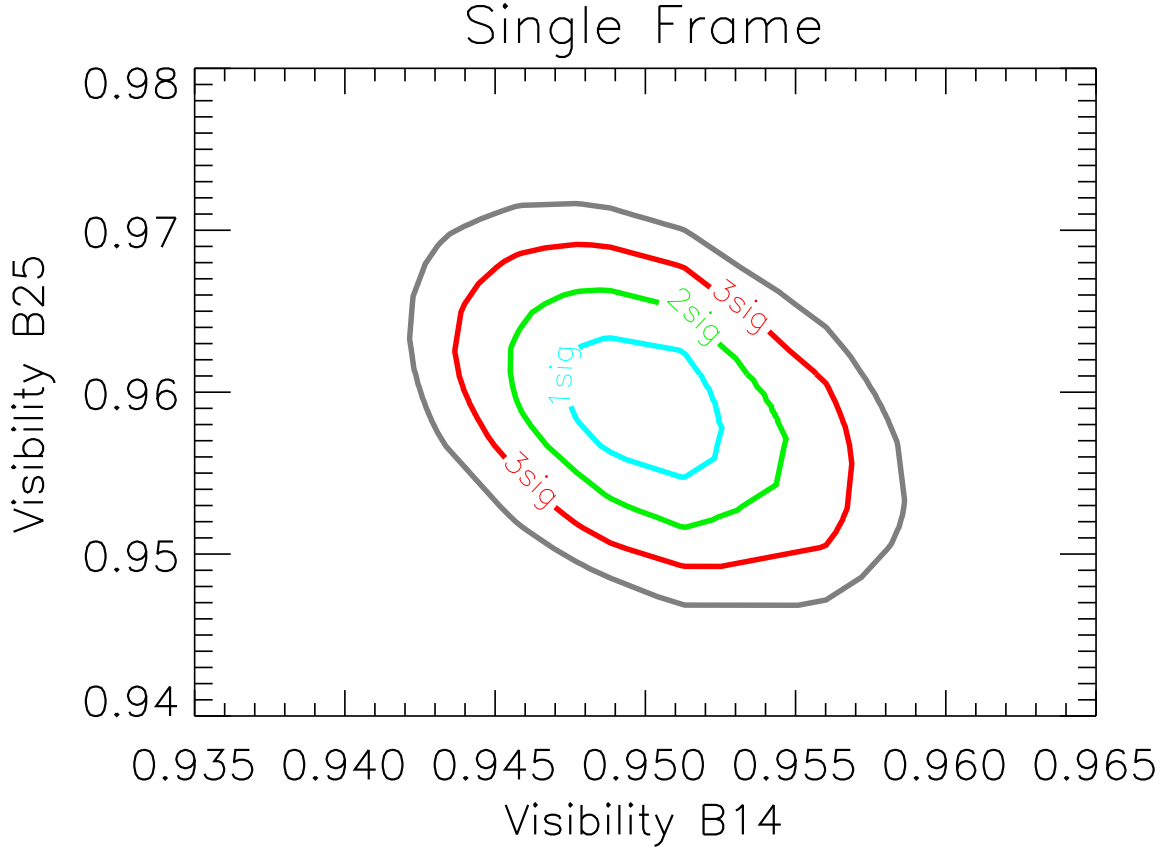
Fig. 11.— A map of \chi^2 space for the correlation between the visibility of beam pair 1-4 and beam pair 2-5, using co-added laser fringes. The confidence intervals correspond to \Delta\chi^2 = \chi^2 - \chi_{\min}^2 = 2.30, 6.17 and 11.8 for 1\sigma, 2\sigma and 3\sigma respectively for 2 parameters of interest (see §4.4, and also Press et al. 2002). The visibility parameters for either beam pair are correlated on the \approx 2\% level for the 3\sigma confidence interval even for these very high signal-to-noise laser fringes. This suggests crosstalk is inherent to the instrument set up.
