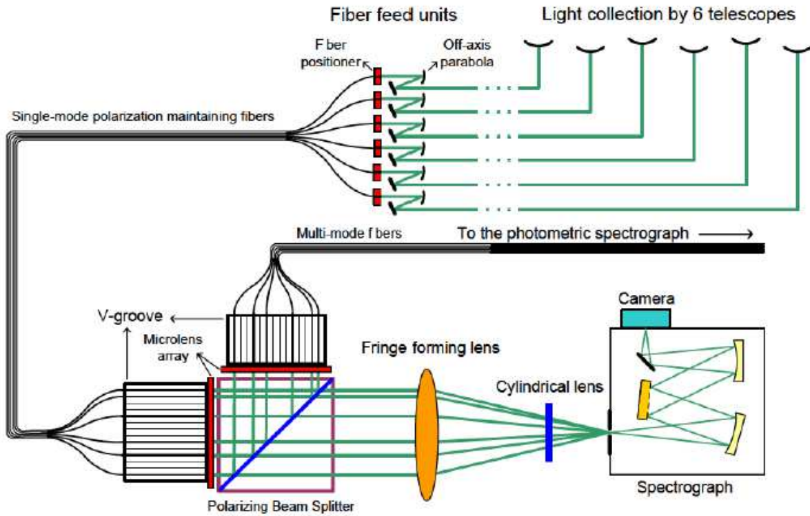
Figure 1. Schematic layout of VISION.
