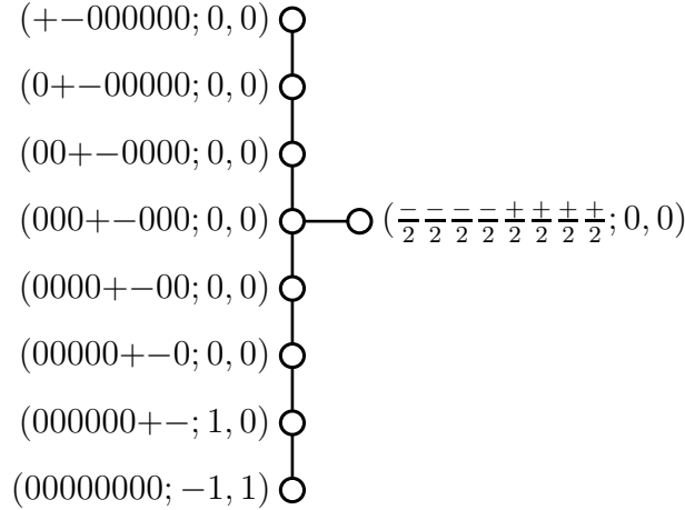
FIGURE 3.1. Simple roots for O^\uparrow(\Lambda)_\nu , where \nu is the root (\frac{\pm}{2} \frac{\pm}{2} \frac{\pm}{2} \frac{\pm}{2} \frac{\pm}{2} \frac{\pm}{2} \frac{\pm}{2}; 00) of \Lambda ; see theorem 3.2.
