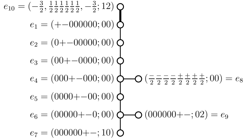
FIGURE 3.2. Simple roots for M = \text{O}^\uparrow(\Lambda)_{\nu, \bar{\rho}} where \rho = (0; 1, 0) and \nu = (\frac{\pm}{2}, \frac{\pm}{2}, \frac{\pm}{2}, \frac{\pm}{2}, \frac{\pm}{2}, \frac{\pm}{2}, \frac{\pm}{2}; 00) ; see the proof of theorem 3.3.
