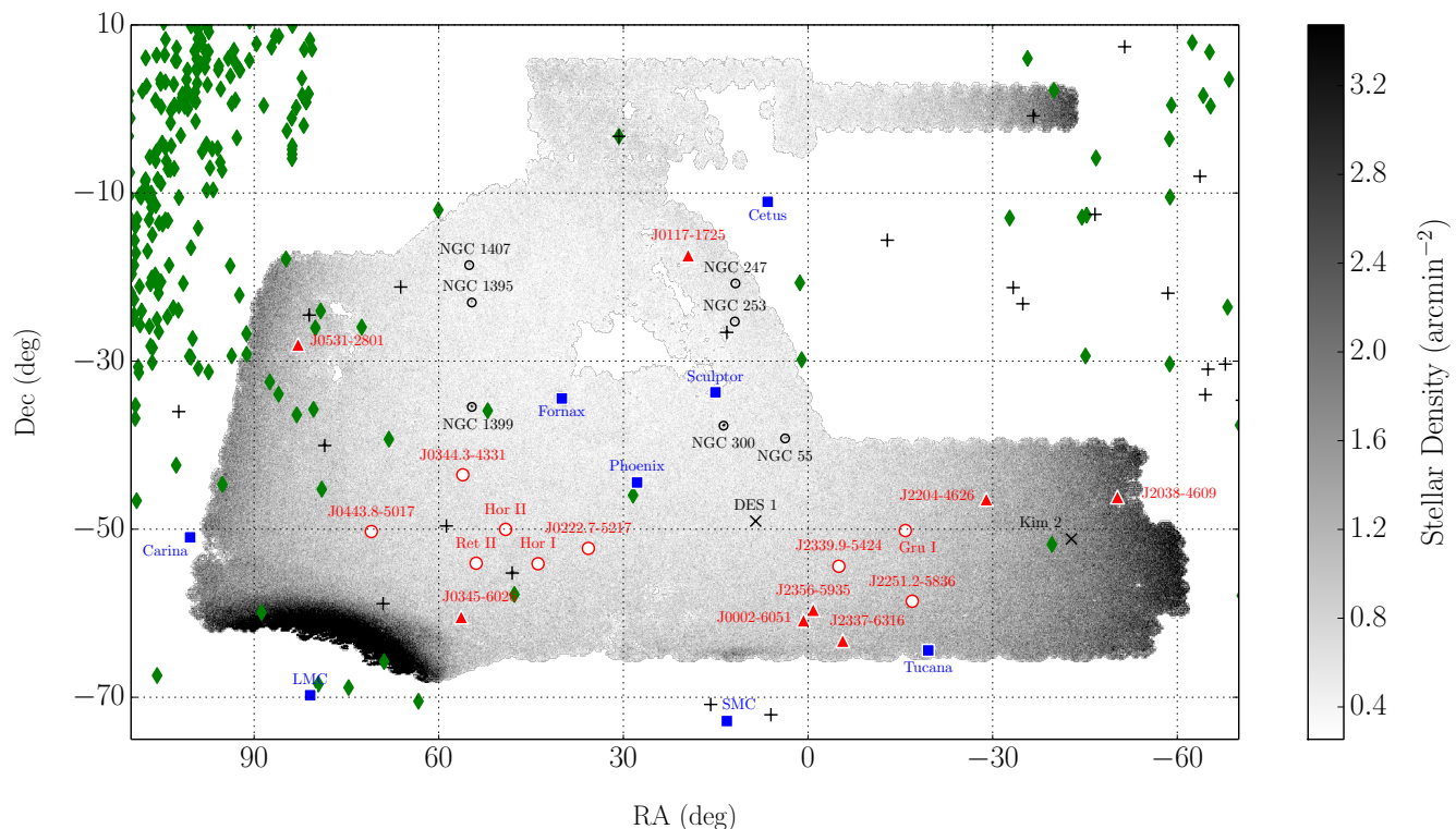
Figure 6. Cartesian projection of the density of stars observed in both g - and r -bands with g < 23 and g-r < 1 over the DES Y2Q1 footprint ( \sim 5000 \text{ deg}^2 ). Globular clusters are marked with “+” symbols (Harris 1996, 2010 edition) two faint outer halo clusters are marked with “x” symbols (Luque et al. 2015), Local Group galaxies known prior to DES are marked with blue squares (McConnachie 2012) dwarf galaxy candidates discovered in Y1 DES data are marked with red outlined circles, while the Y2 stellar systems are marked with red triangles. Open clusters from the WEBDA database are shown as green diamonds. The periphery of the LMC can be seen in the southeast corner of the footprint, while the Galactic stellar disk can be seen on the eastern and western edges. This figure was adapted from Drlica-Wagner et al. (2015b).
