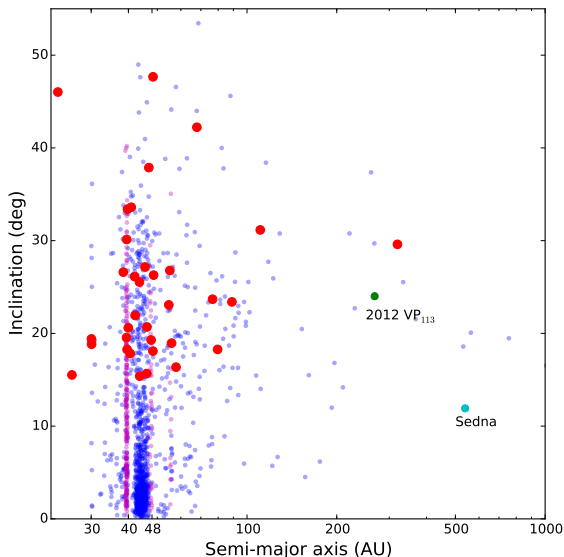
Figure 4. Inclination vs. semi-major axis for 32 distant solar system objects (large circles) discovered in the DES supernova fields. Small circles indicate other known TNOs. The band of objects at a = 39.3 AU are plutinos in a 3:2 mean motion resonance with Neptune. The inner Oort cloud objects Sedna and 2012 VP 113 are also indicated. Due to the location of the search fields, all of the new detections have inclinations of at least 15^\circ .
