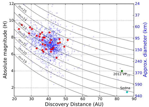
Figure 5. Absolute magnitude vs. heliocentric distance at discovery for 32 distant solar system objects (large circles) discovered in the DES supernova fields. Small circles indicate other known TNOs. The conversion from absolute magnitude to size assumes an albedo of 5%. The inner Oort cloud objects Sedna and 2012 VP 113 are also indicated.
