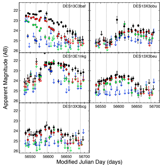
Figure 15. Examples of five hostless SLSNe candidates selected from Y1 of DES. These are in addition to DES13S2cmm (Papadopoulos et al. 2015) which was spectroscopically confirmed. The long multi-colour light curves of these candidates are consistent with other SLSNe and are not AGNs due to the lack of a visible host galaxy. The colours are blue (g-band), green (r-band), red (i-band) and black (z-band). Upper limits are shown as arrows.
