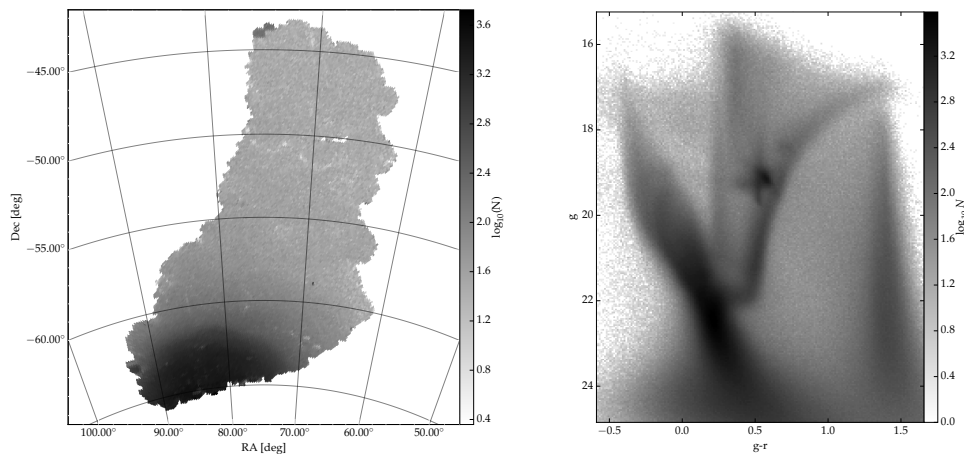
Figure 7. Left: Density map of sources classified as stars in the SPT-E region covered by the DES SV data; Right: g vs. (g-r) Hess diagram of all objects classified as stars and located at DEC < -55^\circ . The LMC main sequence stars (MS) are visible over almost the entire magnitude range. More than one main-sequence turn-off point (MSTO) is present, attesting a large age range which includes an old population with MSTO at (g, g-r) \simeq 22.5, 0.3 . Clear sub-giant and red giant branches (SGB and RGB, respectively) associated with the older populations are also seen redwards of (g-r) \simeq 0.4 for g < 22.3 . The width both at the main sequence and at the RGB attest a significant metallicity spread as well. The red clump and horizontal branches are also clearly visible. The AGB bump is also visible at g = 18.5 and g-r = 0.7 .
