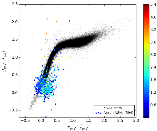
Figure 13. DES gri colour-colour diagram showing the stellar locus as well as known quasars overlapping the DES Science Verification observations. The quasars have been colour-coded according to redshift. While the low redshift quasars overlap the stellar locus, the z > 4 quasars clearly appear as very red ( g - r ) sources.
