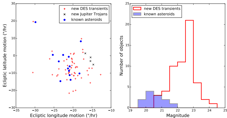
Figure 2. Properties of transients observed in a single visit to the DES supernova search field X3, consisting of five 360-second i -band exposures on 24 Sept 2013. Left: hourly motion in ecliptic latitude and longitude, with objects matched to previously-known main belt asteroids indicated. The new DES detections include several Jupiter Trojans that are among 19 such objects found by DES to date. Right: Comparison of magnitudes of previously-known objects with new DES detections. The known asteroids have a median i -band magnitude of 20.5, compared to a median of 22.6 for the new DES objects.
