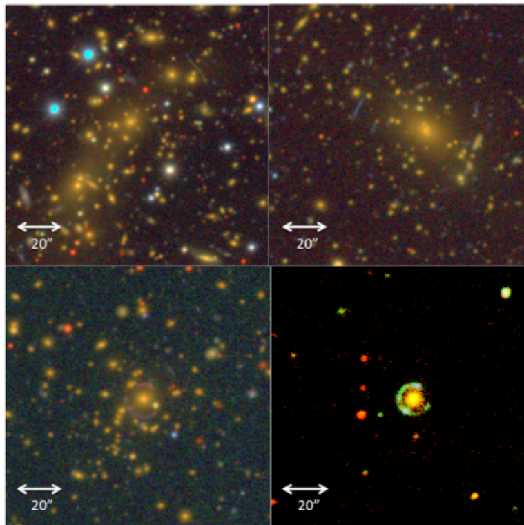
Figure 12. Four examples of known strong lensing systems from DES Science Verification and Year 1 Data.
