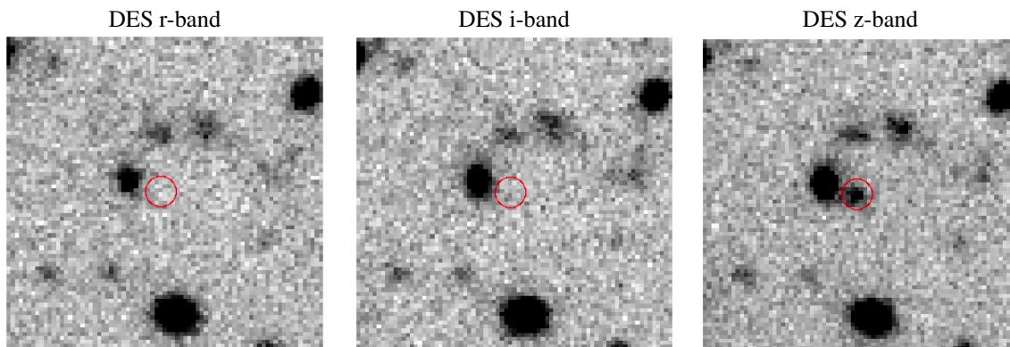
Figure 11. DES r , i and z -band images in the DES deep fields for a spectroscopically confirmed galaxy at z = 6.07 galaxy from Willott et al. (2013). The galaxy position is marked by the red circle in all three images. As can be seen, this high-redshift galaxy is undetected in the DES r and i -bands but detected in the redder DES z -band. This characteristic “drop-out” behaviour of high-redshift galaxies can be exploited to find similar z > 6 galaxies in the DES deep fields.
