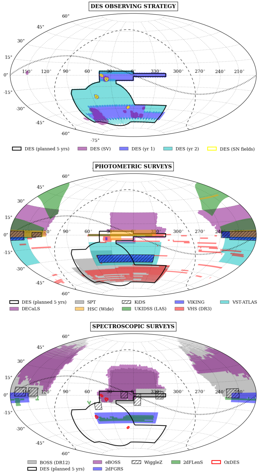
Figure 1. DES and some selected completed or ongoing surveys (as of December 2015). This is a Hammer projection in equatorial coordinates, with the dashed and dotted lines indicate the Galactic plane and the ecliptic plane, respectively. Top: DES survey footprint for the SV, Y1, Y2 and the final 5-yr survey; Middle: with other photometric surveys; Bottom: with other spectroscopic surveys. Planned wide-field surveys not shown include LSST and WFIRST (both photometric), Euclid (photometric and spectroscopic), Sumire PFS, DESI and 4MOST (all three spectroscopic). We note the VHS (DR3) indicates deep coverage in the DES area. Eventually it will cover nearly the whole of the DES 5-yr footprint. A shallower VISTA whole-hemisphere is also underway. The DES footprint was designed to have large overlap with SPT (shown here in the 'photometric surveys' plot). DES SV and Y1 areas essentially completely overlap SPT, and the full planned DES overlaps the completed 2500 sq deg SPT.
