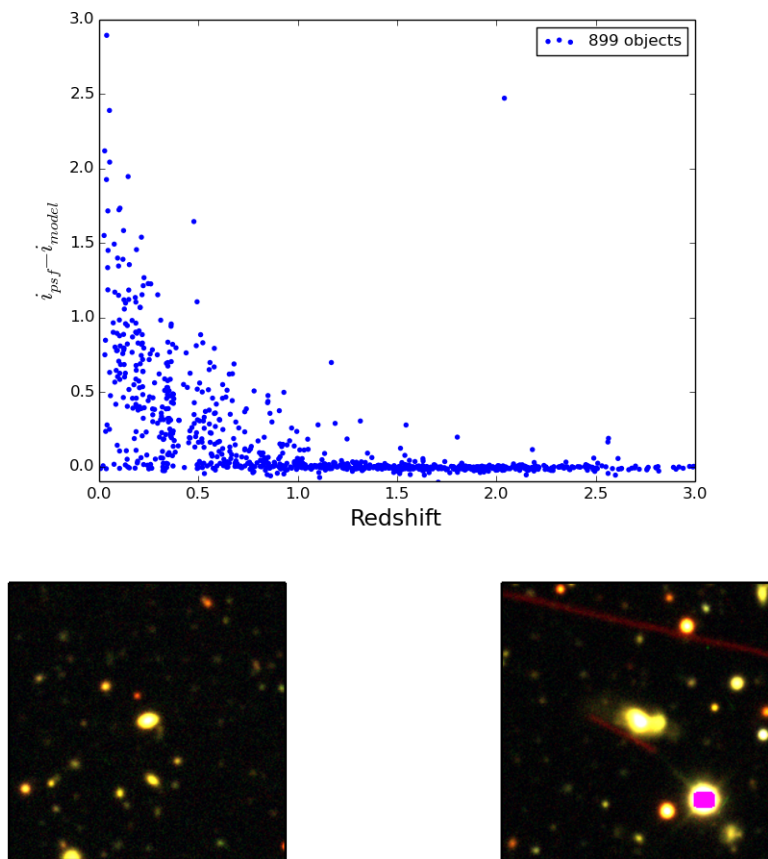
Figure 14. Extended objects can be identified by comparing the psf magnitude to the model magnitude. Top: The figure shows that many quasars in our sample are resolved (appear to be extended objects) even out to z \sim 1.0 . Bottom: DES gri colour-composite images of two known quasars at z = 0.85 (left) and z = 1.17 (right). Both quasars have extended morphologies in the DES data demonstrating that low surface-brightness host galaxy features are clearly visible for quasars out to z \sim 1 .
