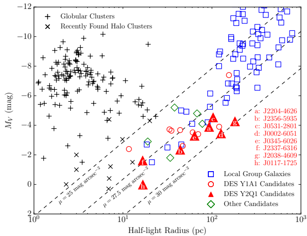
Figure 8. Absolute V-band magnitudes and half-light radii of MW satellites and Local Group dwarf galaxies. MW globular clusters are marked with “+”, fainter clusters and ambiguous objects are marked with “x”, while spectroscopically confirmed dwarf galaxies are marked in blue. The red markers show the new dwarf galaxy candidates found in DES Y1+Y2, while green markers show candidates found in other surveys. Figure taken from Drlica-Wagner et al. (2015c).
