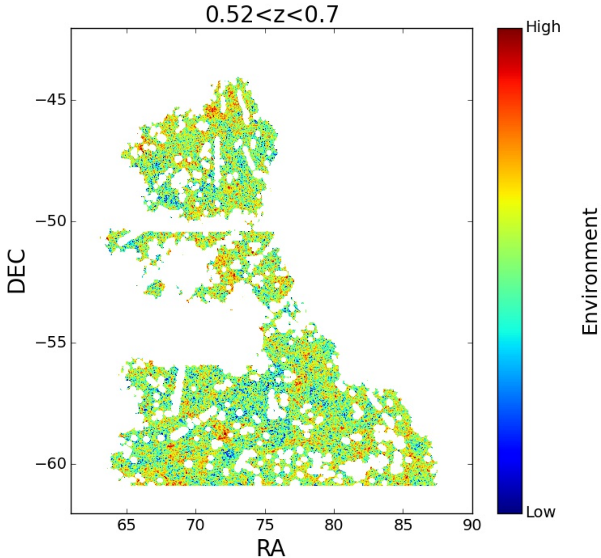
Figure 10. Galaxy environment maps derived from photometric redshifts in a slice at redshift 0.52 < z < 0.70 for a \approx 100 sq deg footprint overlapping with the SPT-E field derived from the DES SV data. Dense environments are shown in red and sparse environments in blue.
