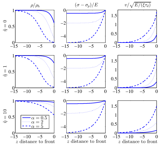
FIG. 4. Typical steady-state profiles of density, stress and velocity along the monolayer. (Online version in colour.)
