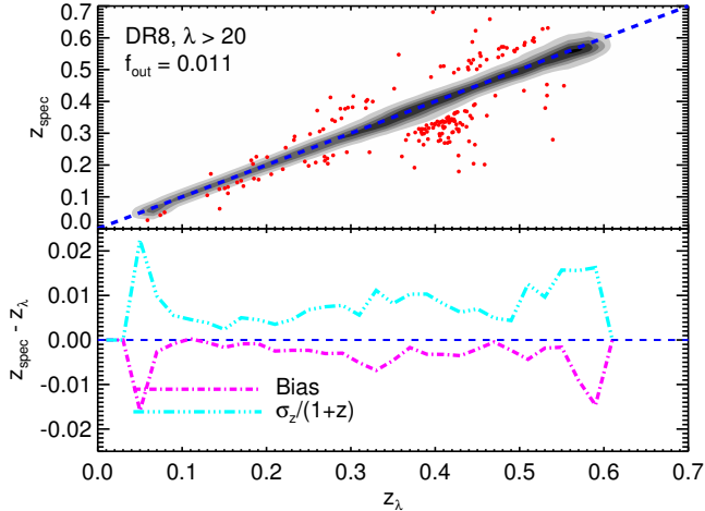
Figure 4. Top: Central galaxy spectroscopic redshift z_{\text{spec}} vs. cluster photometric redshift z_{\lambda} for SDSS DR8 clusters with \lambda > 20 . Grey shaded regions show 1, 2, and 3\sigma density contours. Red points, comprising 1.1% of the total sample, show > 4\sigma outliers. The outlier clump at z_{\lambda} \sim 0.4 is not due to photometric redshift failures, but rather centering failures: these are primarily clusters with a correct photometric redshift, but whose photometrically assigned central galaxy is not in fact a cluster member. Bottom: Bias in z_{\text{spec}} - z_{\lambda} (magenta) and z_{\lambda} scatter \sigma_z/(1+z) (cyan) for clusters with central galaxy spectra. Over most of the redshift range the bias is < 0.005 and the scatter \sigma_z/(1+z) < 0.01 .
