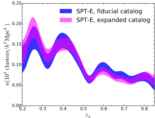
Figure 9. Number density of clusters for the expanded (magenta) and fiducial (blue) catalogs, limited to the SPT-E region. The number density is consistent within 1\sigma at all redshifts in spite of the changes in star/galaxy separation and masking.
