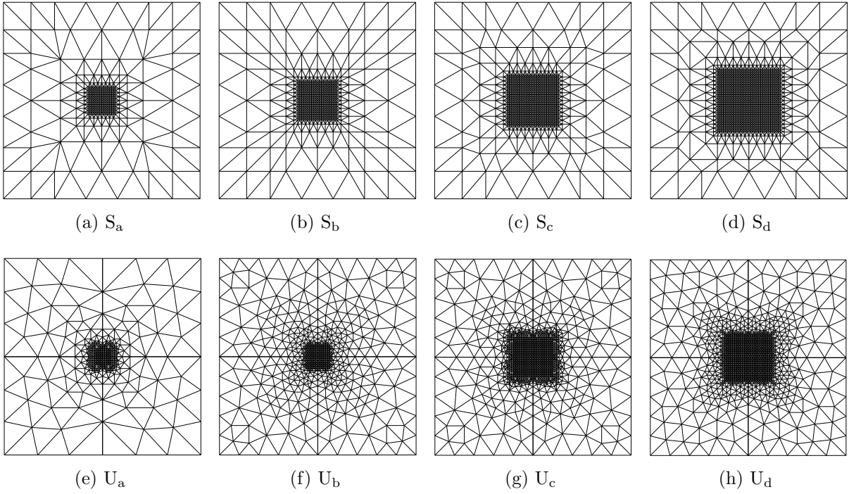
Figure 5: Eight triangulations for the uniaxial loading test: (a) – (d) structured "S" meshes, used also in Beex et al. (2014b) , and (e) – (h) unstructured "U" meshes. The sizes of the fully-resolved regions, the numbers of repatoms, sampling atoms, and sampling bonds corresponding to these meshes are provided in Tab. 2 .
