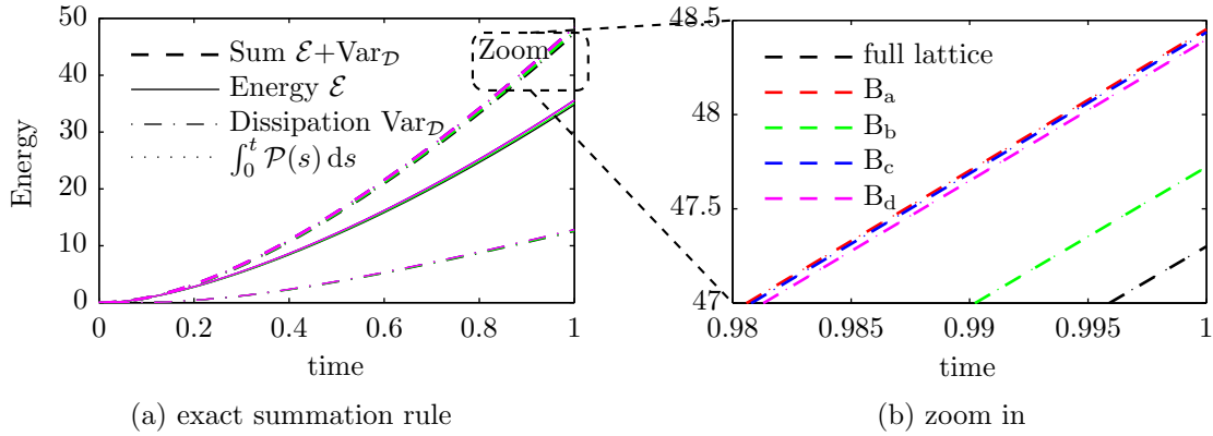
Figure 11: Results for the pure bending test: (a) total energy evolution paths, (b) zoom in; the different meshes from Fig. 10 using exact summation rule are compared to full-lattice solution.
