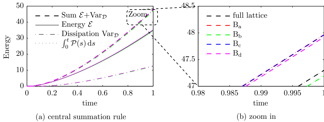
Figure 12: Results for the pure bending test: (a) energy evolution paths, (b) zoom in; the different meshes from Fig. 10 using the central summation rule are compared to full-lattice solution.
