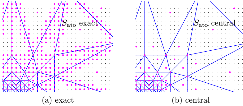
Figure 3: Schematic representation of the two sets of sampling atoms contained in S_{\text{ato}} ; small black dots denote ordinary atom sites and larger magenta dots emphasize the sampling atoms. The triangulation is depicted in the blue colour.
