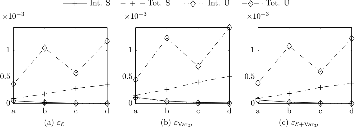
Figure 7: Results for the uniaxial loading test: relative error \varepsilon_{\bar{\square}} (Eq. (40)) for the meshes presented in Fig. 5. "Int." relates to interpolation (exact summation rule) and "Tot." to interpolation plus summation (central summation rule).
