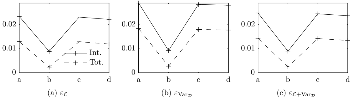
Figure 13: Results for the pure bending test: relative errors \varepsilon_{\square} defined in Eq. (40) for various meshes depicted in Fig. 10. "Int." relates to interpolation (exact summation rule) and "Tot." to interpolation plus summation (central summation rule).
