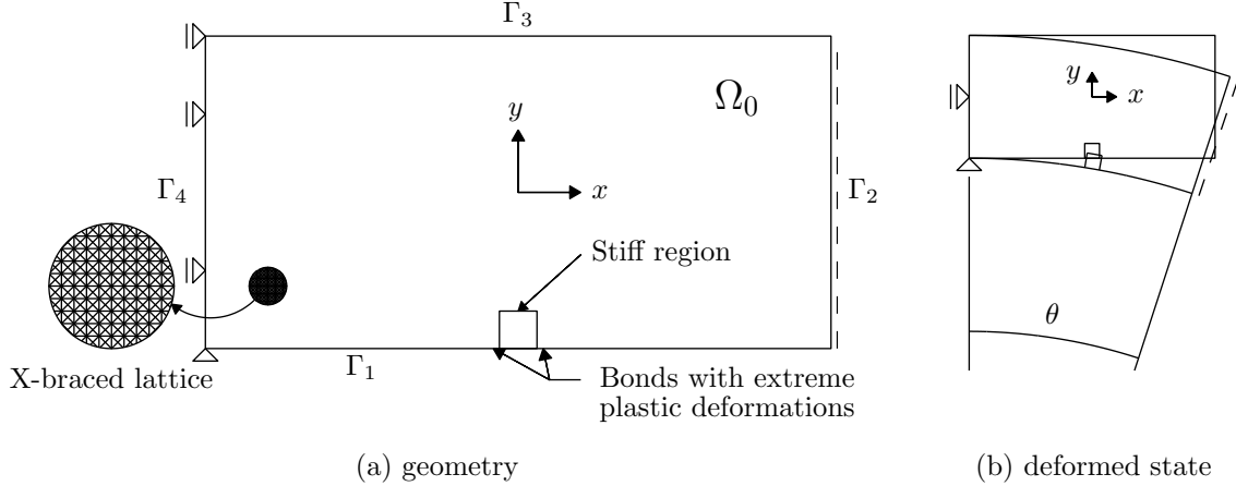
Figure 9: Scheme of the pure bending test: geometry, boundary conditions, and deformed state
