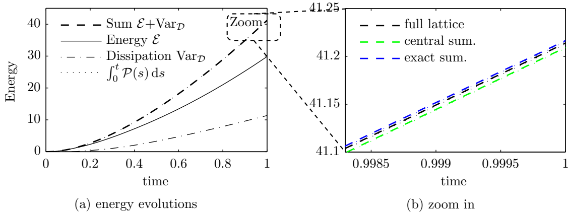
Figure 6: Results for the uniaxial loading test: (a) total energy evolution paths for all meshes and both summation rules, (b) zoom in of only mesh S_a (Fig. 5a) for the exact and central summation rule.
