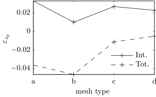
Figure 14: Results for the pure bending test: relative error \varepsilon_{z_p}(t = 1) defined in Eq. (45) for various meshes depicted in Fig. 10. "Int." relates to interpolation (exact summation rule) and "Tot." to interpolation plus summation (central summation rule).
