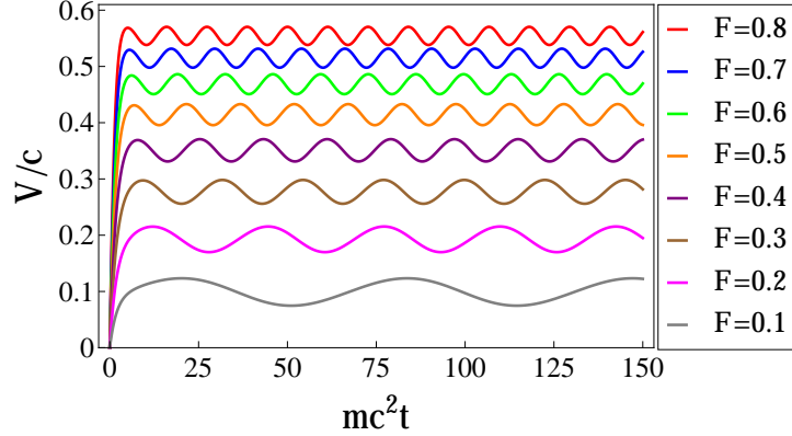
FIG. 3. Schematic velocity as a function of time for various forces listed in the legend ( F in units of F_{\text{max}} = 2nmc^2 ). As F increases, the drift velocity and frequency of oscillations increases.
