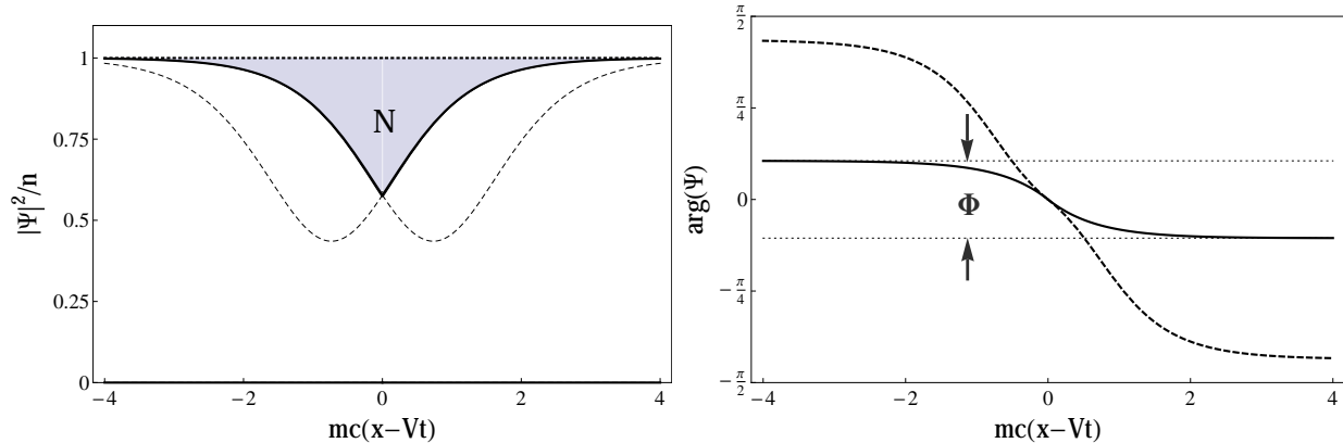
FIG. 5. Solution of Eq. (31) obtained by matching two grey solitons. Left panel: the density profile. Right panel: the phase profile. The collective variables N and \Phi are shown.
