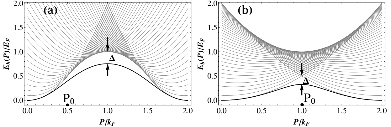
FIG. 6. (Color online) The bound-state E_b(P) , Eq. (42), (thick black line) and scattering continuum \frac{(P-k)^2}{2M} + E_h(k) for a set of k (thin gray lines) for the light impurity M/m = 1/2 (a) and heavy impurity M/m = 2 (b). In both cases mG/n = 0.7 .
