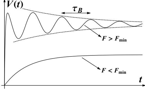
FIG. 4. Schematic noise-averaged velocity as a function of time including the effects of fluctuations. For F < F_{\min} the impurity velocity saturates below the critical velocity and Bloch oscillations do not occur. For F_{\min} < F < F_{\max} Bloch oscillations occur, but are attenuated in time due to dephasing, see Eq. (24).
