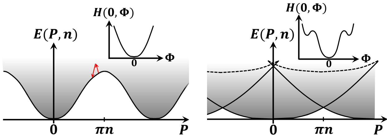
FIG. 2. Schematic dispersion relation for a mobile impurity in a 1D quantum liquid. Left panel: When the impurity mass is subcritical M < M_c the dispersion is smooth, and the energy function H(P, \Phi) has a unique minimum at \Phi(P) . At low temperatures, two-phonon scattering processes (red arrows) lead to energy and momentum relaxation of the impurity. Right panel: For M > M_c the groundstate develops singular cusps at odd integer multiples of \pi n , and the function H(P, \Phi) acquires metastable minima (the dashed lines in E(P, n) represent local maxima of H(P, \Phi) ).
