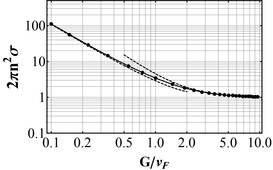
FIG. 7. Nonlinear mobility for the equal mass impurity in a Tonks-Girardeau gas. The dashed lines are the asymptotic limits given by Eq. (46).
