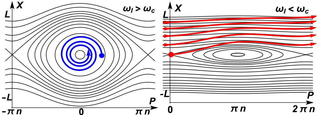
FIG. 8. (Color online) Impurity trajectory in a trapped quantum liquid. The black curves represent schematic constant energy contours of Eq. (51). Left panel: for \omega_I > \omega_c the adiabatic orbits are stable in the vicinity of the energy minimum at (X, P) = (0, 0) . Impurity acceleration leads to phonon damping and thus a decreasing energy and oscillation amplitude (thick blue curve). Right panel: for \omega_I < \omega_c ( \omega_I = 0 shown) the orbits are instead stable near the energy maximum (X, P) = (0, \pi n) . In the case of strong coupling, the maximal displacement on the separatrix orbit is much smaller than the trap size L . In this case the impurity escapes by radiating phonons in the running momentum phase (here P is plotted modulo 2\pi n ), where the velocity exhibits Bloch oscillations plus drift (thick red curve).
