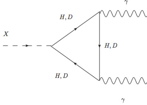
Figure 3: The new singlet scalar/pseudoscalar X \equiv \theta_{34} with mass 750 GeV is decays into a pair of photons due to its coupling to a loop of vector-like fermions D, \bar{D} which are colour triplets and have electric charge \mp 1/3 .
