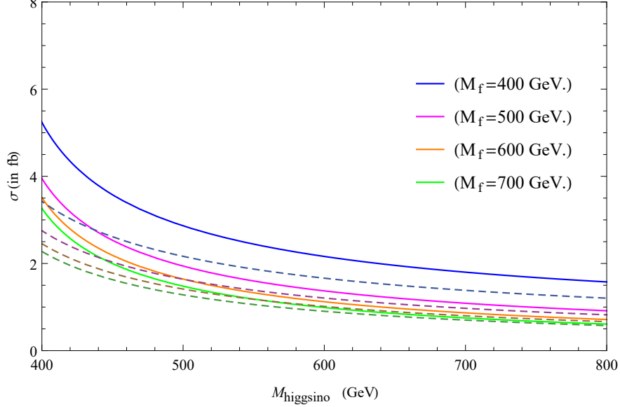
Figure 4: The cross section \sigma(pp \rightarrow X \rightarrow \gamma\gamma) (in fb units) in the parametric space of the Higgsinos H_u^j/H_d^j , for a selection of masses of the vector-like D_i/\bar{D}_i with all masses M_i set equal to M_f and the coupling y_f . The solid lines correspond to the Pseudoscalar candidate state, while the dashed lines of the same hue correspond to the Scalar option.
