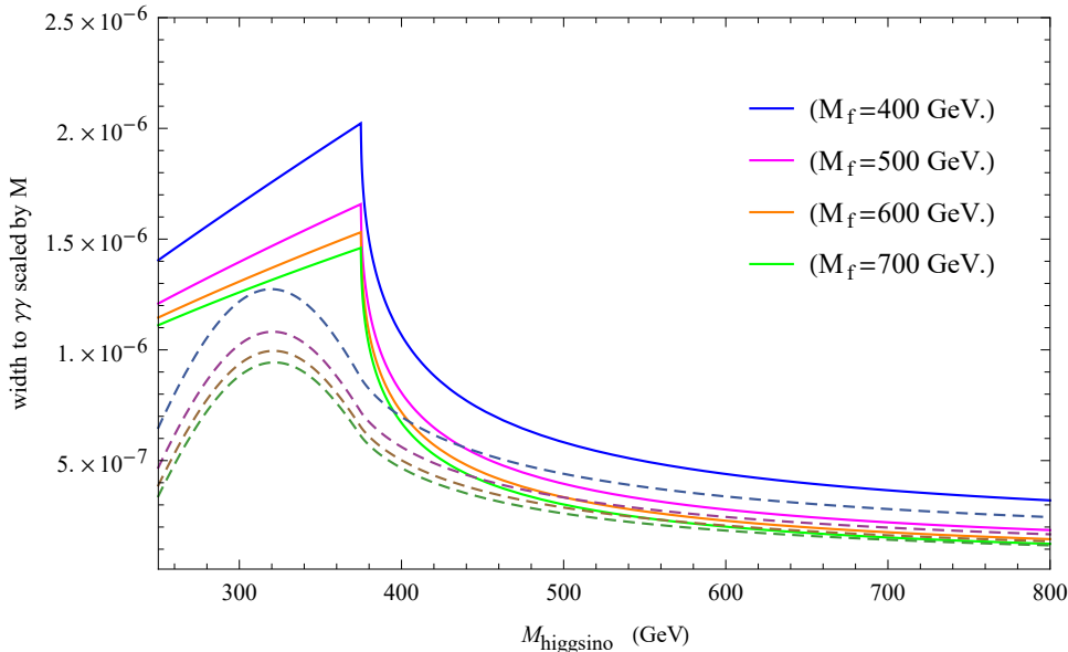
Figure 5: The mass weighted width \Gamma(X \rightarrow \gamma\gamma) in the parametric space of the Higgsinos H_u^j/H_d^j , for a selection of masses of the vector-like D_i/\bar{D}_i with masses M_f and the coupling y_f . The solid lines correspond to the Pseudoscalar candidate state, while the dashed lines of the same hue correspond to the Scalar option.
