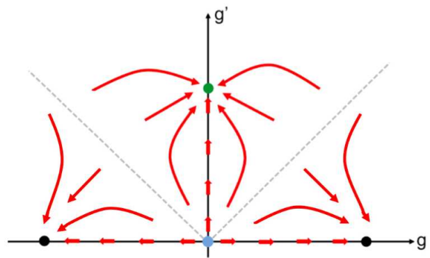
FIG. 6. RG flow chart. g is the strength of O_2 and g' is the inter-copy coupling strength. The red arrows are the RG flow and the grey line is the phase boundary.
