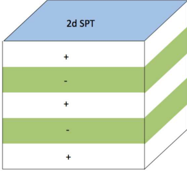
FIG. 3. The slab configuration of PDW. the green/white slab contains pairing strength with positive/negative sign. The nodal plane(blue) contains a 2d SPT state.
