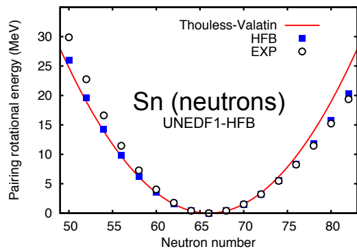
FIG. 1. (Color online). Neutron pairing rotational energy measured from a reference state in ^{116}\text{Sn} . The parabolic expression (1) with \lambda_n and \mathcal{J}_{nn} evaluated for the reference nucleus is shown as a solid line. The HFB (squares) and experimental (circles) values have been extracted from binding energies according to E_{\text{rot}}^{\text{pair}} = E(N) - E(66) - \lambda_n(66)(N - 66) .
