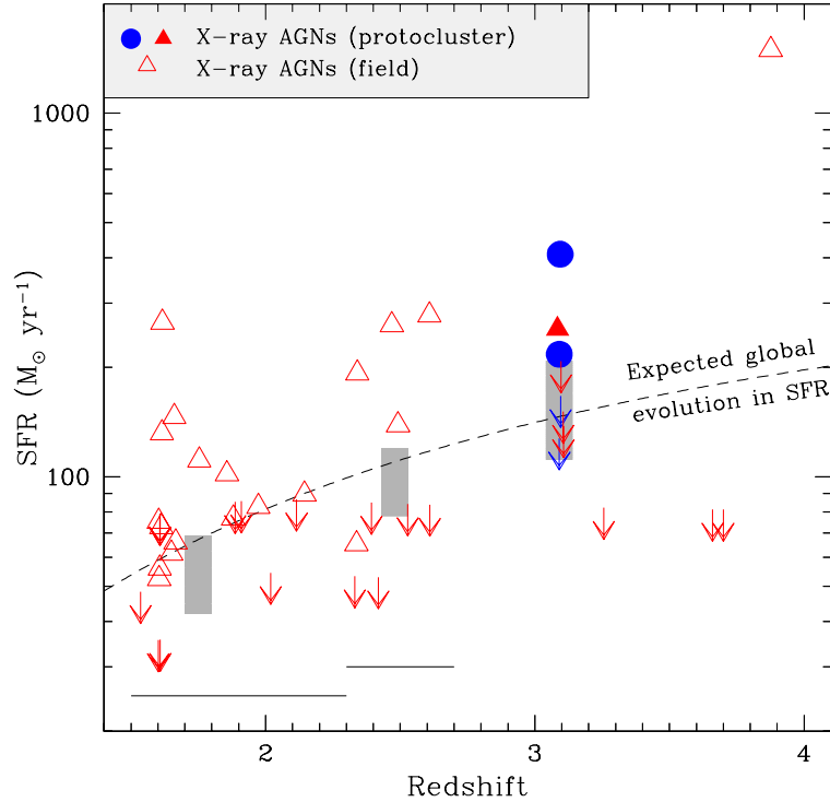
Figure 3. Infrared luminosity from star formation versus redshift for the X-ray detected AGNs in the SSA 22 protocluster compared with X-ray detected AGNs in the field (open triangles; taken from Mullaney et al. 2015); see Fig. 1 for the other symbol descriptions. The conversion from L_{\text{IR}} to SFR is calculated using Eqn. 1. The shaded regions indicate the range in mean infrared luminosities for the protocluster AGNs at z \approx 3.09 and for the AGNs in the field at two mean redshifts; the redshift ranges are indicated by the grey horizontal lines. The widths of the shaded regions are arbitrary. The dashed curve indicates the measured evolution in infrared luminosity for an M_* star-forming galaxy over z = 1.4\text{--}4.1 from Schreiber et al. (2015), using the definition of M_* from Ilbert et al. (2013). There is significant scatter in the infrared luminosities for individual X-ray AGNs; however, the mean infrared luminosities are consistent with M_* star-forming galaxies at the average redshifts for both the protocluster and field AGN samples.
