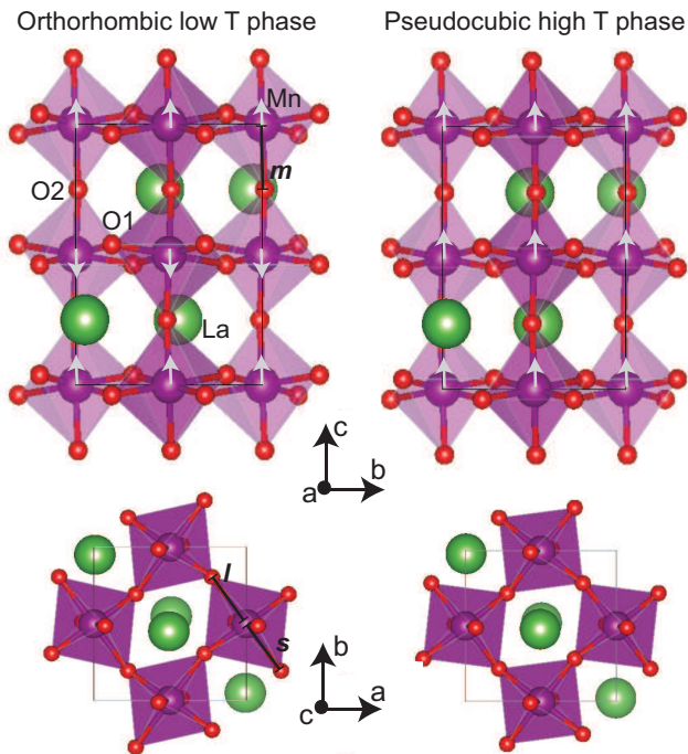
FIG. 1. Side and top views of the orthorhombic low T phase (left) and the pseudo-cubic high T phase (right) of \text{LaMnO}_3 structure. Long ( l ), medium ( m ), and short ( s ) Mn-O bonds as well as the spin ordering are shown.
