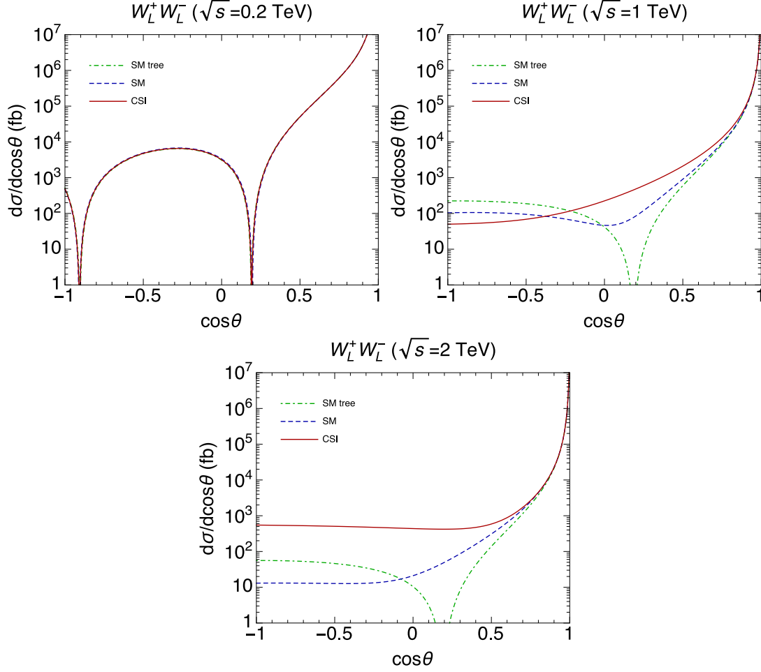
Figure 6: Differential cross sections for W_L^+ W_L^- \rightarrow W_L^+ W_L^- process for the c.m. energies \sqrt{s} = 0.2 TeV, 1 TeV and 2 TeV. We set N = 1 . \theta represents the angle between the initial W^+ and final W^+ momenta in the c.m. frame. See text for the input parameters. (a) Dot-dashed (green) line represents the Born SM cross section, (b) dashed (blue) line the SM cross section, and (c) solid (red) line the CSI model cross section.
