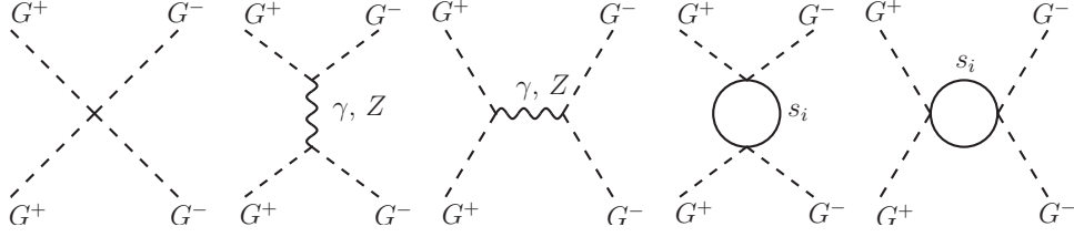
Figure 11: Diagrams for G^+G^- \rightarrow G^+G^- scattering. (Time flows upwards.) The last two diagrams are the new contributions in the CSI model.
