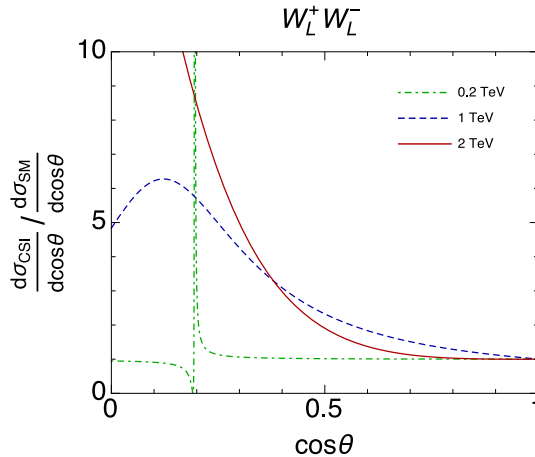
Figure 7: Ratio of the W_L^+ W_L^- scattering differential cross sections for the CSI model and SM vs. \cos\theta , at \sqrt{s} = 0.2 TeV (green dot-dashed), 1 TeV (blue dashed) and 2 TeV (red solid).
