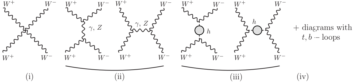
Figure 4: Diagrams for W^+W^- \rightarrow W^+W^- scattering. Time flows upwards.
