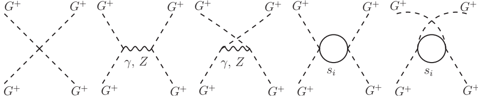
Figure 12: Same as Fig. 11 but for G^+G^+ \rightarrow G^+G^+ scattering.
