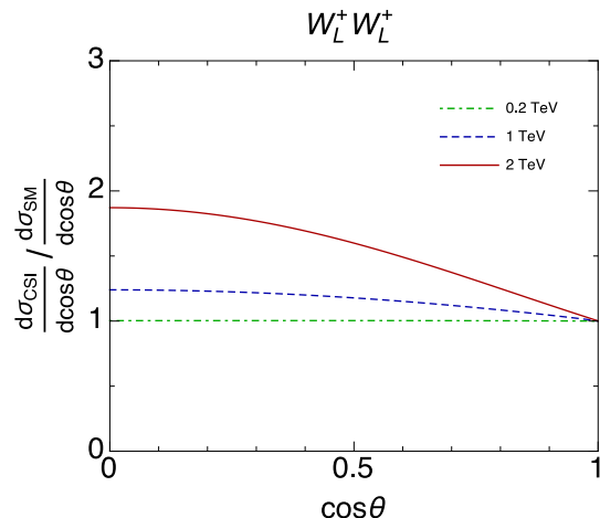
Figure 9: Same as Fig. 7 but for W_L^+ W_L^+ scattering.
