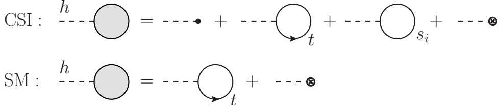
Figure 1: Higgs tadpole diagrams in the CSI model and the SM. A blob in the CSI model represents the tree-level vertex, while a vertex with cross represents the counterterms. (The counterterms in the CSI model and the SM are different. See text.)
