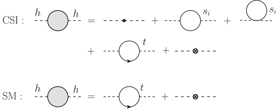
Figure 2: Higgs self-energy diagrams in the CSI model and the SM. Similarly to Fig. 1, a blob and a vertex with a cross represent the tree-level vertex and counterterm, respectively.
