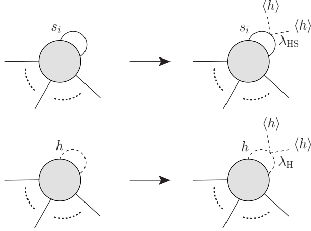
Figure 10: Insertion of \lambda_{\text{HS}}v^2s_i s_i vertex to a 1PI diagram, and insertion of \lambda_{\text{H}}v^2hh vertex to a 1PI diagram, respectively. These manipulations do not increase the number of loops.
