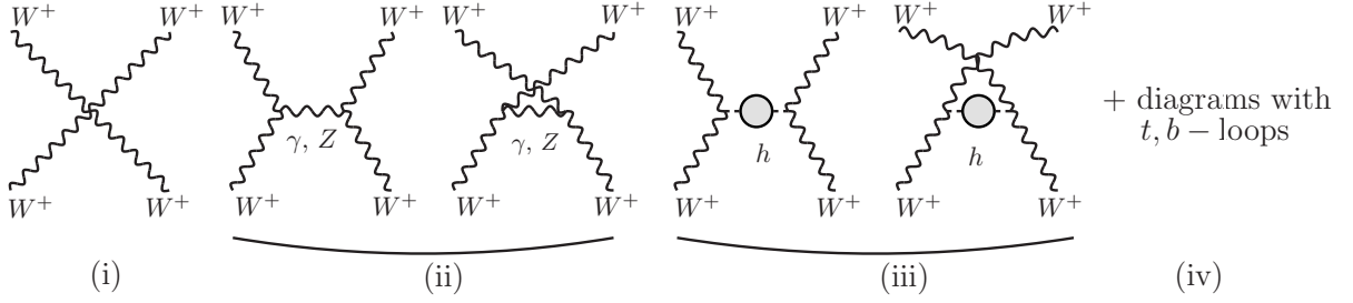
Figure 5: Diagrams for W^+W^+ \rightarrow W^+W^+ scattering. (Time flows upwards, which is similar to Fig. 4.)
