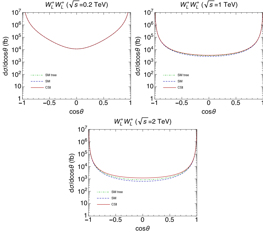
Figure 8: Same as Fig. 6 but for W_L^+ W_L^+ \rightarrow W_L^+ W_L^+ process.
