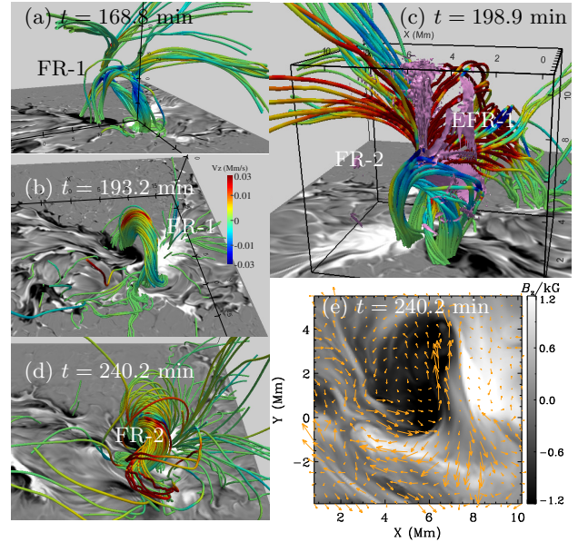
FIG. 5. (a)–(d) Magnetic field lines coloured by the vertical velocity at times indicated to illustrate the formation and eruption of two flux ropes (FR). The field lines traced in (c) pass through the current-layer iso-surface (pink) with a value J/B = 1/4\delta z , where J is the current density. (e) Horizontal velocity vectors in the \delta -sunspot region. The grey shaded surface represents the vertical magnetic field at z = 0 . A fly-by animation of panel (c) also including the sub-surface structure of the \delta -sunspot is available at http://www.mn.uio.no/astro/english/people/aca/piyali/fluxemerge/fig5c.mp4 . Also available is an animation of the time evolution of the magnetic field in this region at http://www.mn.uio.no/astro/english/people/aca/piyali/fluxemerge/fig5pr1.mp4 .
