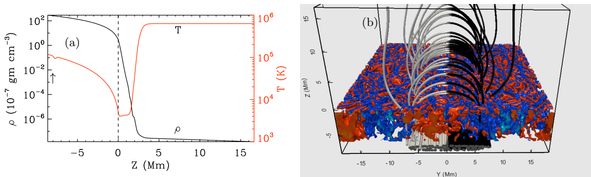
FIG. 1. (a) Vertical profiles of the horizontal averages of initial density and temperature. The arrow indicates the position of the cool magnetic sheet. (b) Initial magnetic field-lines shaded black (white) indicating positive (negative) B_z . The iso-surfaces of the upward (red) and the downward (blue) velocity in the convective layer highlights the granulation pattern.
