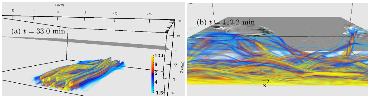
FIG. 2. Volume rendering of the quantity B\rho^{-1/4} . The gray shaded surface represents B_z in the z = 0 layer.
