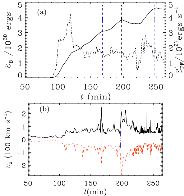
FIG. 4. Evolution of (a) magnetic energy, \mathcal{E}_B (solid), and \dot{\mathcal{E}}_{PF} (dashed-dotted) and that of (b) maximum positive (solid) and negative values (dashed) of vertical velocity above the active region. The three vertical lines denote the times of the two flares and a flux rope eruption respectively.
