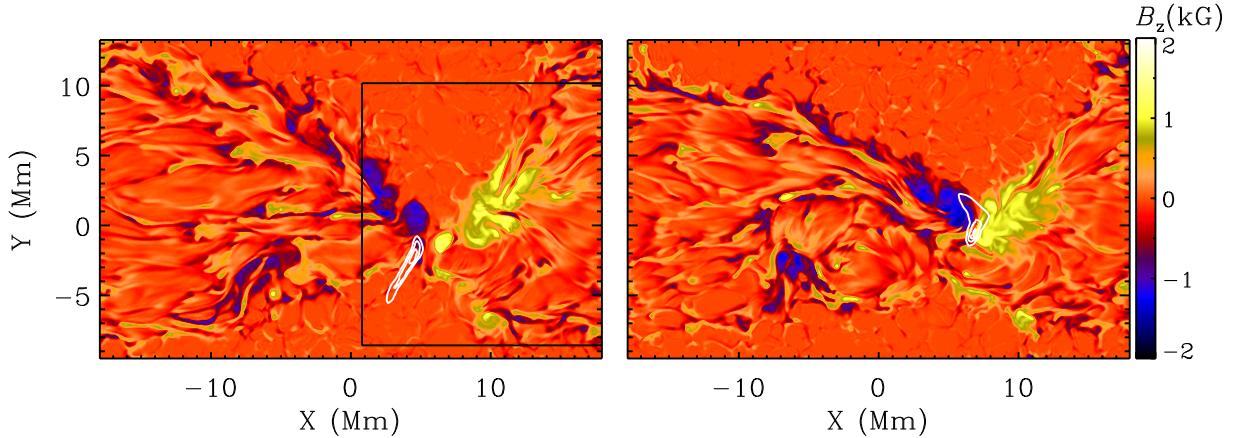
FIG. 3. Vertical component of the magnetic field, B_z , at z = 0 (shaded contours) at times indicated. Overlaid line contours (white) in (a) represent temperature contour levels at z = 3.26 Mm for values 90,000K, 1MK, 1.2MK whereas the respective temperature contour levels in (b) are at 90,000K, 1MK, 2.2MK. This figure is available as an animation at http://www.mn.uio.no/astro/english/people/aca/piyali/fluxemerge/fig3pr1.mp4 .
