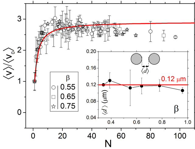
FIG. 3. (Color online) Normalized average speed \langle v \rangle / \langle v_0 \rangle of colloidal worms as a function of the number of rotors N for different ellipticity \beta ( \omega = 62.8 \text{ rad s}^{-1} , H_0 = 2300 A m^{-1} ). Points denote experimental data while the continuous line is a fit following Eq.(1). Inset shows the average surface distance \langle d \rangle vs \beta .
