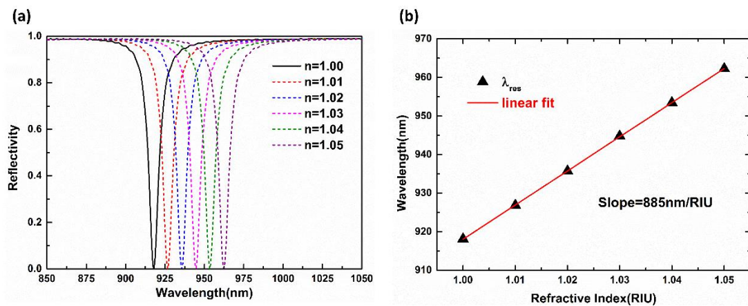
Fig. 4 (a) Reflection spectrum of the all-metal perfect absorber with the refractive index varying from 1 to 1.05 with a step interval of 0.01. (b) Resonant wavelength as a function of the surrounding low refractive index. The red line is the linear fitting with the slope representing the sensitivity S .
