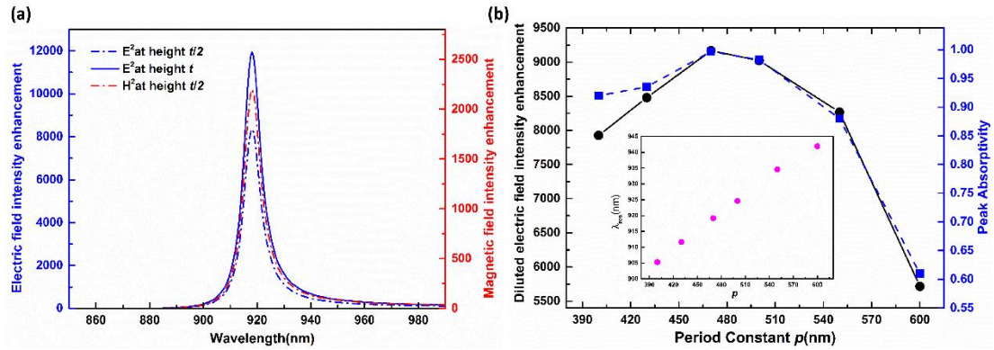
Fig. 3 (a) Electric (blue dash-dot curve) and magnetic field (red dash-dot curve) intensity enhancement at a point in the middle of the gap and height t/2 over the silver film, and electric field intensity enhancement at height t (blue curve). (b) Diluted electric field intensity enhancement (circles connected with solid lines) and the peak absorptivity (squares connected with dashed lines) as the period varies. Inset: resonant wavelength vs period with other parameters unchanged.
