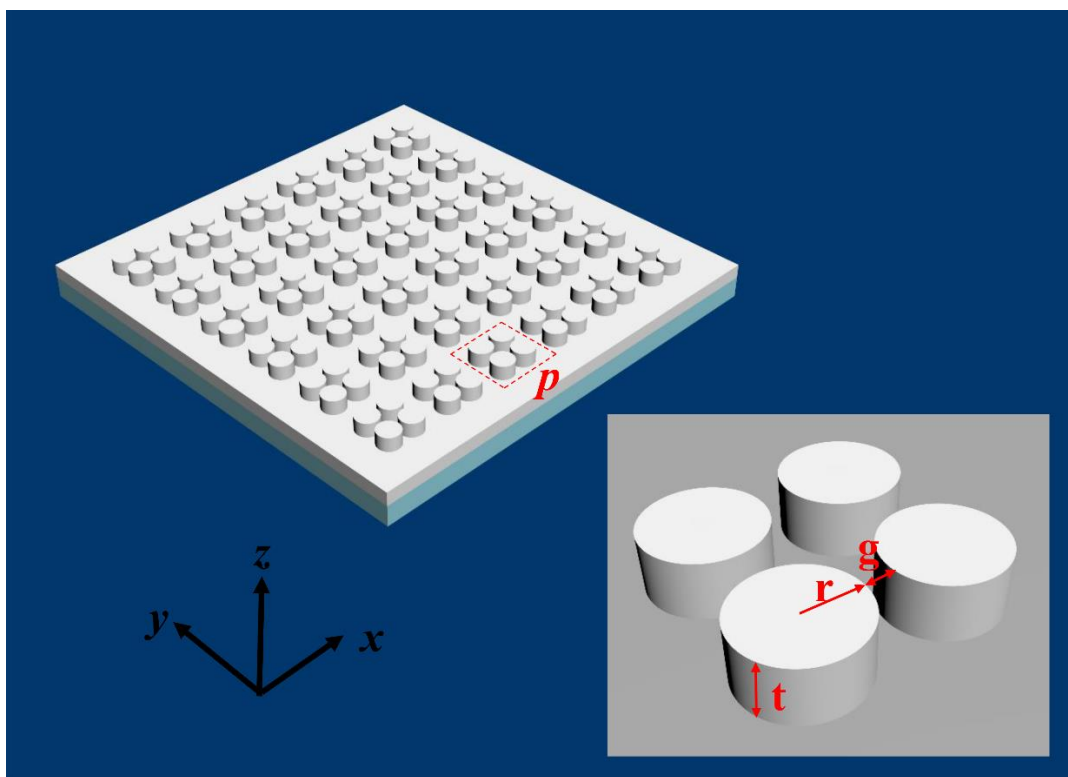
Fig. 1 A schematic diagram of the all-metal perfect absorber with a magnified unit cell (enclosed in dashed box) shown in the inset: periodic arrays of coupled thick silver disks are placed directly on the surface of a uniform silver film. The closely spaced silver disks have a radius ( r ) of 80nm , thickness ( t ) of 100nm and gap distance ( g ) of 20nm . The period constant ( p ) of the arrays is 470nm and the bottom silver film has a thickness of 100nm . In addition, the whole structure is placed on a glass substrate, and the surrounding material is assumed to be air.
