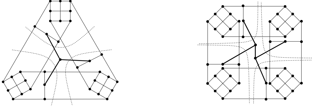
(b) Blowup( Prism, C_4 ) [12, Figure 7].
