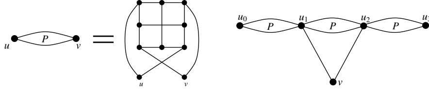
Figure 8: The 2-pole P_{u,v}^- and the subgraph described in Lemma 6.3.
