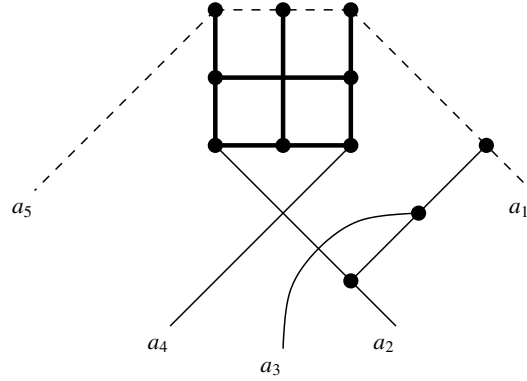
Figure 12: An illustration to the proof of Theorem 7.7. Edges of the circuit are shown dashed, edges of X are shown bold.
