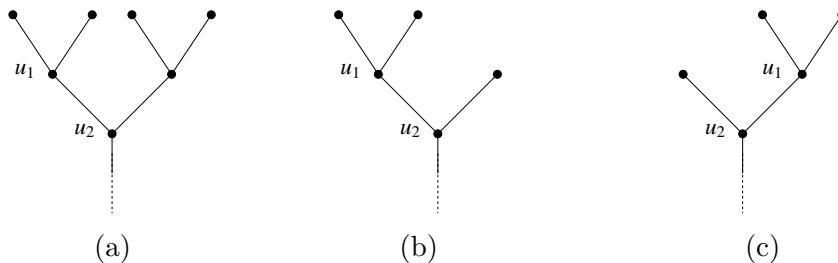
Figure 6: Possible cases in the proof of Theorem 5.1. Any vertex represented as a leaf is a leaf of T_0 .
