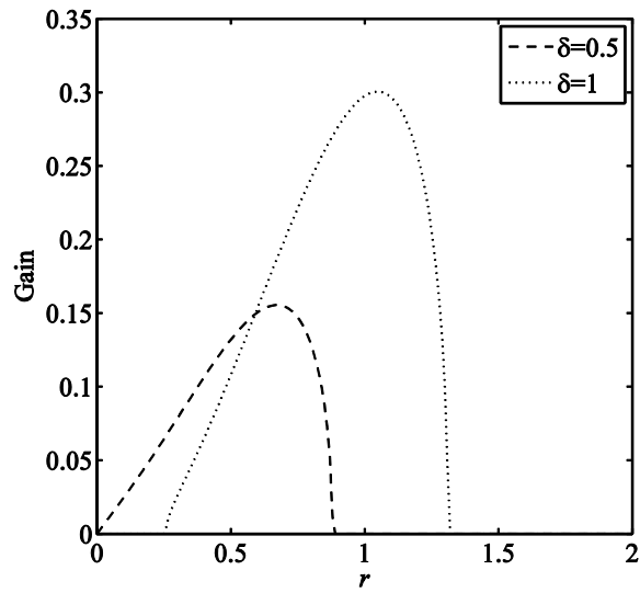
Figure 4: The spectrum of modulation instability gain for S = 1.1 , \Gamma = 1 , \delta = 0.5 and 1 .
