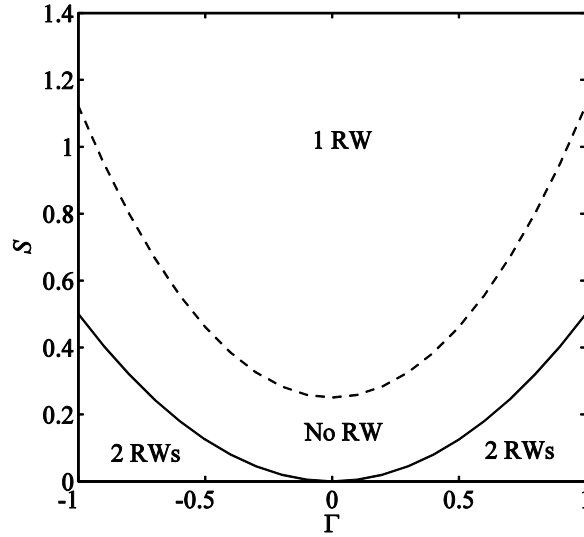
Figure 2: The existence region of RW (rogue wave) in the plane of S (the strength of the defocusing cubic nonlinearity, see Eq. (4)) and \Gamma (the strength of the self-steepening nonlinearity) for \delta = 1 and \rho = 1 . Above the dashed curve ( S = R ) and below the solid line ( S = \Gamma^2/2 ), RWs exist. Between the dashed and solid curves, RWs do not exist.
