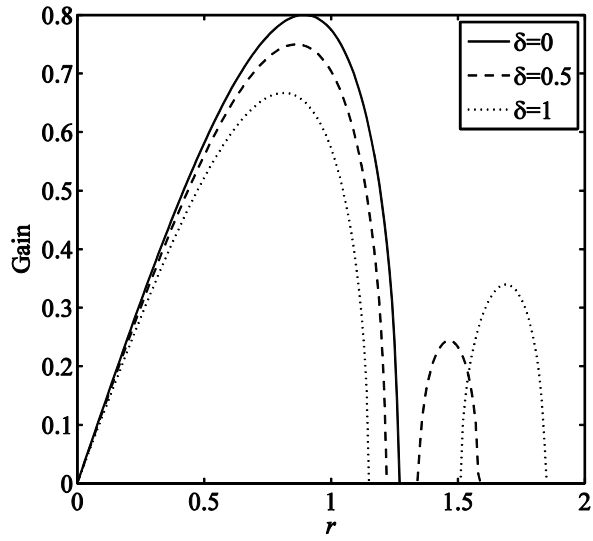
Figure 3: The spectrum of modulation instability gain for S = 0.1 , \Gamma = 1 , and \delta = 0, 0.5, 1 .
