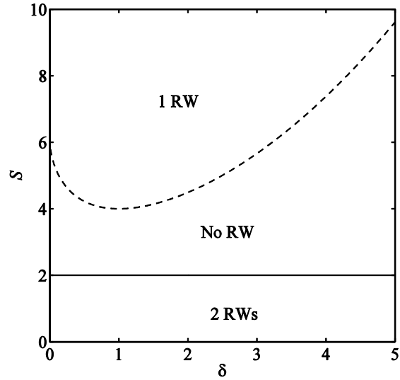
Figure 1: The existence region of RW (rogue wave) in the plane of parameters S (the strength of the defocusing cubic nonlinearity, see Eq. (4)) and \delta (group-velocity mismatch) for \gamma = 2 and \rho = 1 . Above the dashed curve ( S = R ) and below the solid line ( S = \Gamma^2/2 ), RWs exist. Between the dashed and solid boundaries, RWs do not exist.
