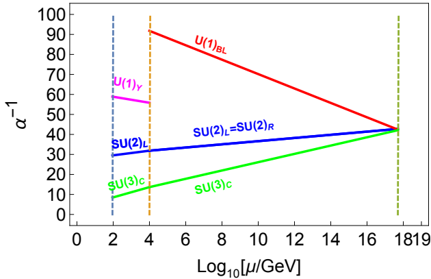
FIG. 1: Gauge coupling running in the considered model accommodating the diphoton excess, demonstrating successful gauge unification at the scale M_{\text{GUT}} = 10^{17.55} GeV with an intermediate left-right symmetry breaking scale at 10 TeV.
