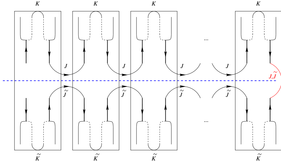
FIG. 10. (Color online) Unfolding a chain of dominoes coupled by time-reversal symmetric interactions.
