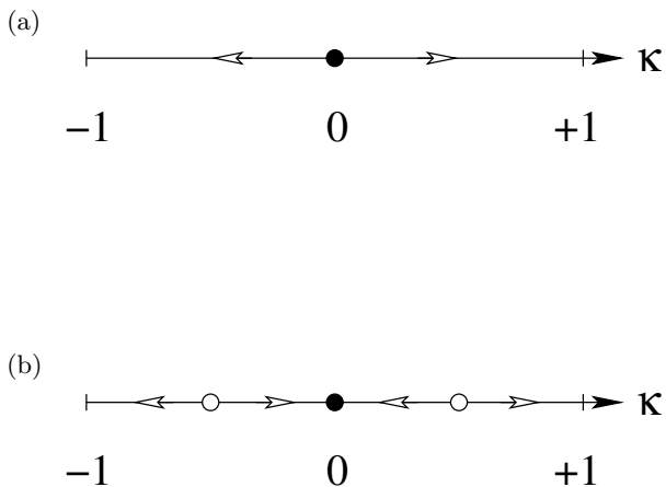
FIG. 7. For the case when the phases transition in the range -1 \leq \kappa \leq +1 are continuous, the critical point at \kappa = 0 is either unstable or stable depending on whether the number of critical points for -1 < \kappa < 0 is even as in (a) or odd as in (b), respectively. [The calculations in Appendix C3 suggest the scenario (a).]
