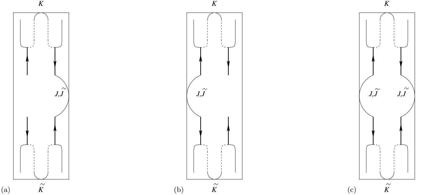
FIG. 9. The partial gapping of a single domino with local current-current interactions can be done in two ways (a) and (b). The complete gapping of a single domino with local current-current interactions is achieved in (c).
