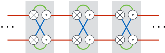
FIG. 1. (Color online) Schematic representation of the Hamiltonian for a state with non-Abelian topological order arising from interactions between electronic quantum wires. Each \otimes and \odot represents the right-moving and left-moving (spinful) electrons of a quantum wire coming out of the plane of the page. Each gray area represents an interaction that gaps out charge fluctuations on the bundle of wires that it encloses. Each line represents a SU(2) symmetric Heisenberg interaction between the spin densities of left-movers and right-movers that it connects. Lines of the same color represent interaction terms of the same strengths.
