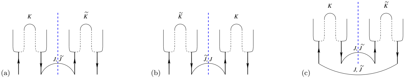
FIG. 11. The partial gapping of a bundle made of 2(k + k') quantum wires with local current-current interactions can be done in two ways (a) and (b). The complete gapping of a bundle made of 2(k + k') quantum wires with local current-current interactions is achieved in (c). The dashed vertical line is a mirror axis of symmetry.
