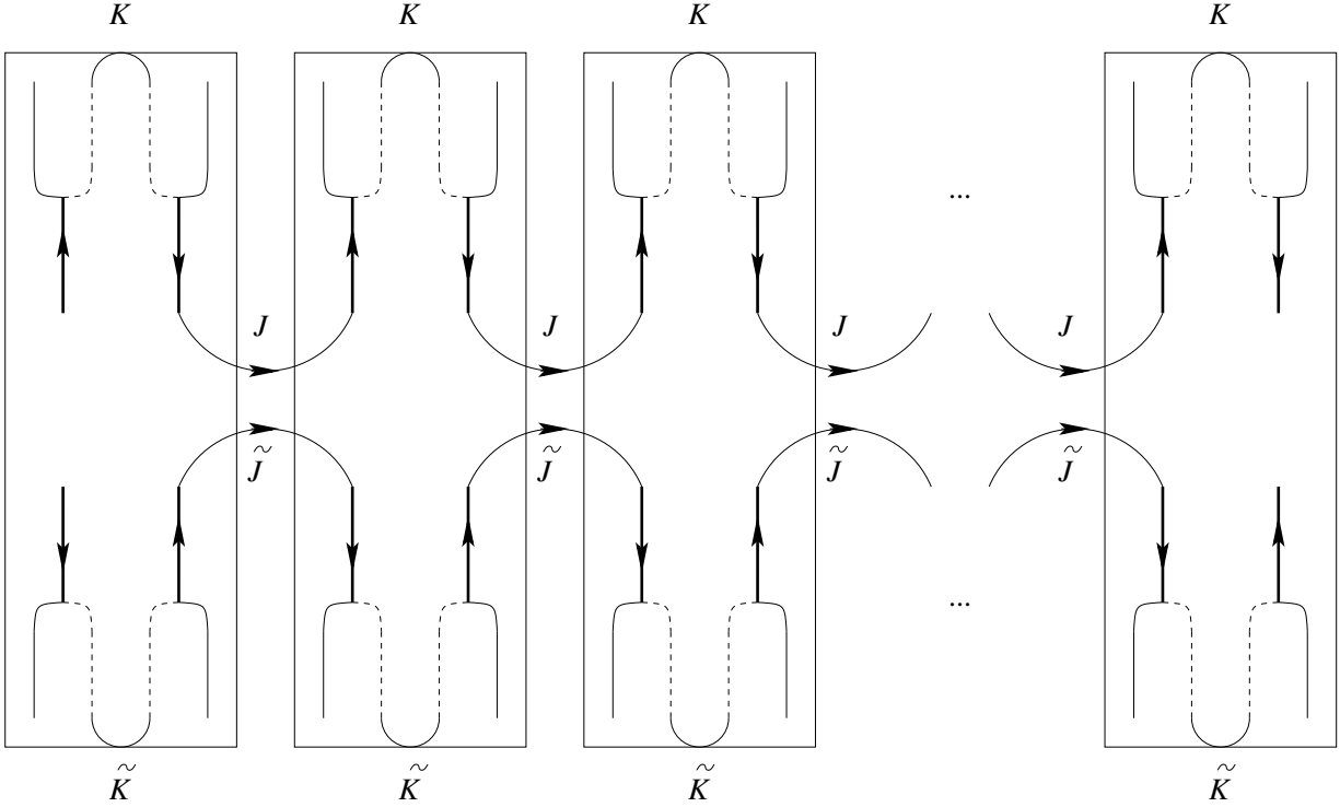
FIG. 8. Chain of N wires, each wire supporting four right- and four left-moving flavors, that are coupled by current-current interactions in a way that is explicitly symmetric under reversal of time. A bundle of 8 \times (k + k') right- or left-moving electronic degrees of freedom is represented by a domino. There are n = N/(k + k') dominoes. The currents denoted by J generate the affine Lie algebra \widehat{su}(2)_k \oplus \widehat{su}(2)_{k'} . The currents denoted by K generate the affine Lie algebra \widehat{su}(2)_{k+k'} . The currents denoted by \tilde{J} generate the affine Lie algebra \widehat{su}(2)_k \oplus \widehat{su}(2)_{k'} . The currents denoted by \tilde{K} generate the affine Lie algebra \widehat{su}(2)_{k+k'} .
