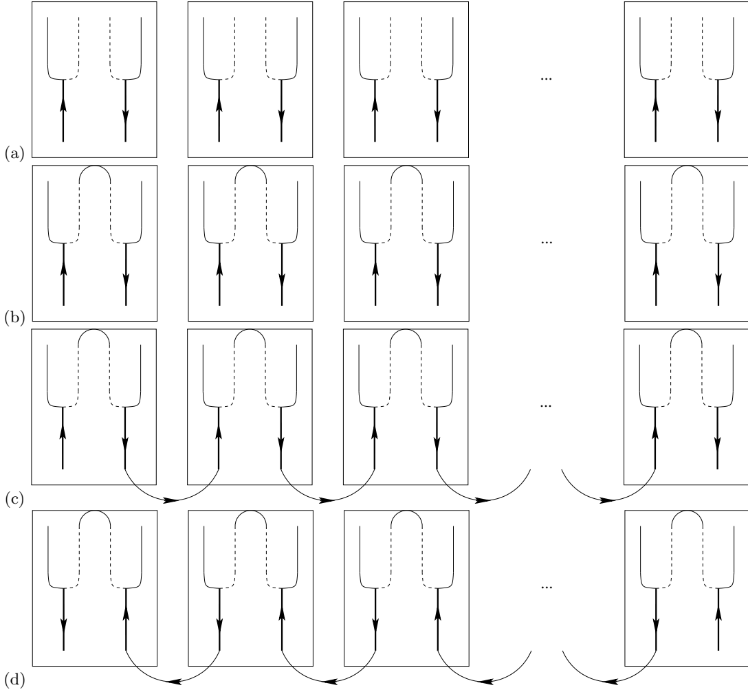
FIG. 5. (a) A chain of wires is partitioned into bundles. A bundle is depicted by a domino. The pattern in the domino corresponds to a right- and left-moving critical sector with the affine Lie algebra \hat{g}_{k,k'} := \widehat{su}(2)_k \oplus \widehat{su}(2)_{k'} represented by a thick vertical line supporting an up arrow for right movers and down arrow for left movers. Its diagonal subalgebra \hat{h}_{k,k'} := \widehat{su}(2)_{k+k'} is represented by the forking into a dashed line. The coset \hat{g}_{k,k'}/\hat{h}_{k,k'} is represented by the forking into a full line. (b) An arc inside each domino depicts a current-current interaction between the generators of \hat{h}_{k,k'} . These arcs gap all the critical modes generated by \hat{h}_{k,k'} := \widehat{su}(2)_{k+k'} within a bundle. (c) An arc between two consecutive dominoes depicts the current-current interactions between the generators of \hat{g}_{k,k'} . The arrows on these arcs indicate that these interactions break time-reversal symmetry. These arcs gap all remaining critical modes except for the modes generated by the right-moving \hat{g}_{k,k'}/\hat{h}_{k,k'} on bundle m = 1 and the modes generated by the left-moving \hat{g}_{k,k'}/\hat{h}_{k,k'} on bundle m = n . (d) Reversal of time is represented by reversing all arrows.
