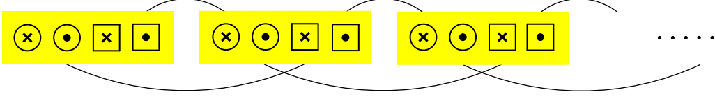
FIG. 13. (Color online) Pictorial representation for the selected backscattering in the symmetry class C. Each yellow box represents a quantum wire composed of four-Majorana degrees of freedom. The wires are enumerated by I = 1, \dots, N in ascending order from left to right. For any I , the Majorana modes are denoted by \chi_{R,+I} , \chi_{L,+I} , \chi_{R,-I} , and \chi_{L,-I} reading from left to right, respectively.
