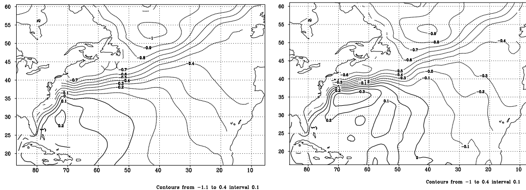
Figure 2: The sea surface height in the North Atlantic on January 30, 2006 computed using the classical (A) and optimized (B) discretization of operators of vertical diffusion at bottom points.
