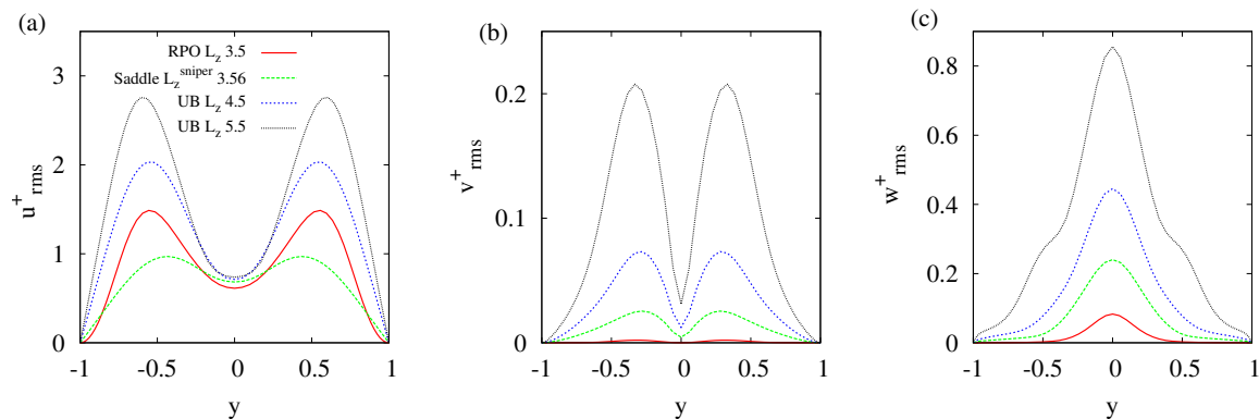
Figure 7. Comparison of the rms velocity profiles of the travelling-wave upper branch solutions for selected values of L_z to the rms profiles of the relative periodic orbit solutions existing for L_z < L_z^* .
