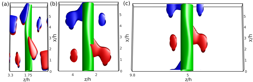
Figure 4. Flow fields associated to the travelling-wave solutions corresponding to the: (a) saddle node L_z \approx 3.55 (X symbol in figure 3), while (b) and (c) are the lower branch solution respectively computed for L_z = 5.55 (empty square symbol in figure 3) and L_z = 10.5 (empty triangle symbol in figure 3). The iso-surfaces at u^+ = -2 are plotted in green, while red and blue surfaces correspond to positive and negative streamwise vorticity at \omega_x = \pm 0.65 \max(\omega_x)
