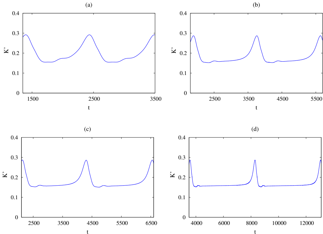
Figure 1. Perturbation energy associated to the relative periodic orbit solutions computed with the edge-tracking procedure for the selected increasing values of the spanwise size L_z = 3.525 , L_z = 3.535 , L_z = 3.540 , L_z = 3.548 (panels a to d ). The initial transient before the convergence to the edge state is discarded. Remark the increasing period of the solutions as L_z is increased.
