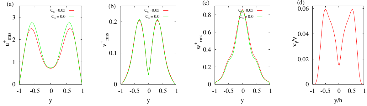
Figure 9. Comparison of the rms velocity profiles of the TW upper branch solutions for C_s = 0 and C_s = 0.05 (with L_z = 5.55 and Re = 2000 ). In panel (d) is displayed the eddy viscosity \nu_t/\nu associated to the subgrid motions modelled in the solution of the filtered (LES) equations at C_s = 0.05 .
