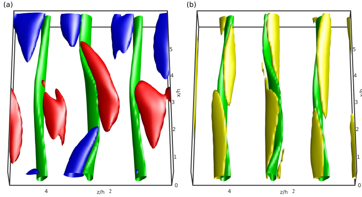
Figure 8. Flow field associated to the upper branch solutions of the filtered (LES) equations computed at L_z = 5.55 for C_s = 0.05 . The iso-surfaces at u^+ = -2 are plotted in green. In panel (a) red and blue surfaces correspond to positive and negative streamwise vorticity at \omega_x = \pm 0.65 \max(\omega_x) , while in panel (b) the yellow surface corresponds to \nu_t/\nu = 0.065 .
