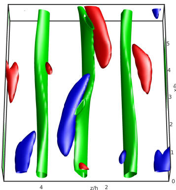
Figure 6. Flow field associated to the upper branch solution computed at L_z = 5.55 corresponding to the filled square symbol in figure 3. The iso-surfaces at u^+ = -2 are plotted in green, while red and blue surfaces correspond to positive and negative streamwise vorticity at \omega_x = \pm 0.65 \max(\omega_x)
