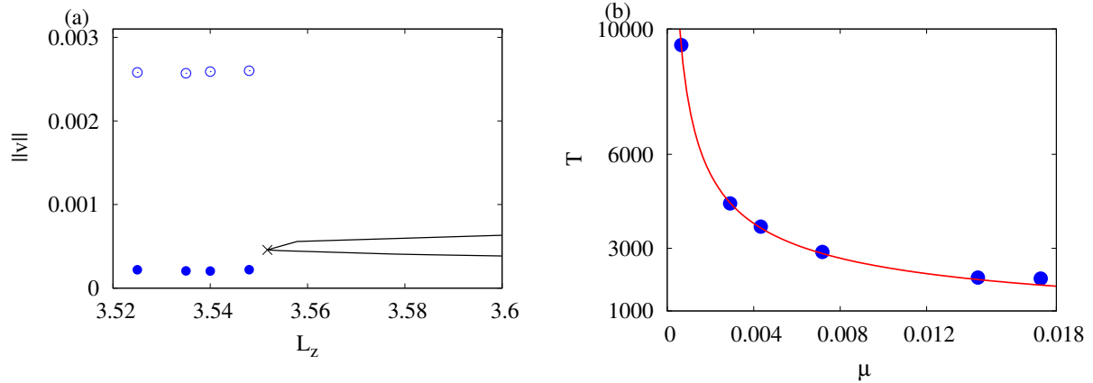
Figure 2. (a) Bifurcation diagram in L_z , with L_x = 2\pi and Re = 2000 where the relative periodic orbit solution disappears in a global saddle-node infinite period bifurcation originating a pair of travelling-wave solutions. The periodic solution is reported with its maximum (empty symbols) and minimum (filled symbols) values of the spatially-averaged wall-normal velocity. The symbols correspond to the L_z values considered in figure 1. The point where the upper and lower branch travelling-wave solutions are generated is denoted by the X symbol. (b) Variation of time period T close to the bifurcation point. The function T \approx 240/\sqrt{\mu} (solid line), where \mu = (L_z^* - L_z)/L_z^* , fits well the data (symbols). The four leftmost symbols correspond to the time-series reported in figure 1.
