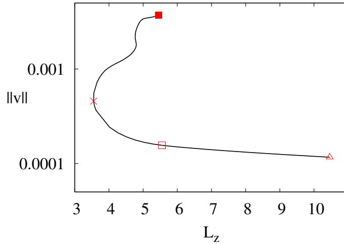
Figure 3. Continuation diagram for travelling-wave solutions as a function of L_z , with L_x = 2\pi and Re = 2000 . The left-most part of the diagram is already reported in figure 2(a). The turning point where the upper and lower branch of the travelling-wave solution originate corresponds to the saddle-node infinite period global bifurcation.
