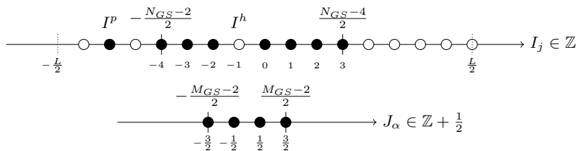
Figure 6: Integer configuration for the particle-hole excitation, explicit numbers for L = 16 , N_{GS} = 10 , M_{GS} = 5 .
