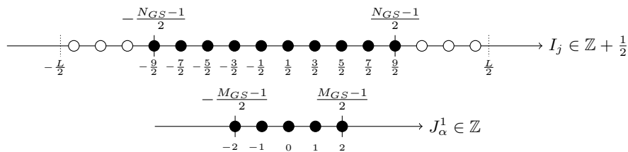
Figure 1: Configuration of the integers for the ground state, explicit numbers given are for L = 16 , N_{GS} = 10 , M_{GS} = 5
