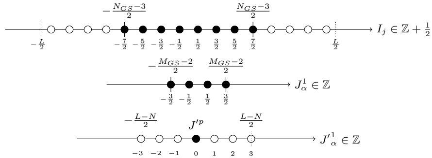
Figure 4: Configuration of the integers for the k - \Lambda string excited state
