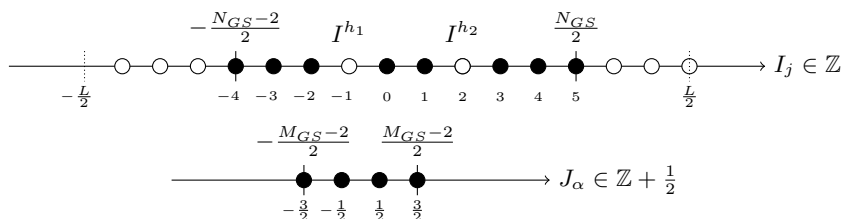
Figure 10: Integer configuration for two hole excited state, explicit numbers for L = 16 , N_{GS} = 10 , M_{GS} = 5 .
