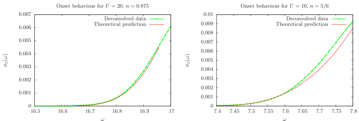
Figure 17: Comparison of deconvolved DMRG data with the onset as predicted in (103), varying the offset and overall scale factor and choosing \Lambda = (1 - n)\pi/10 .
