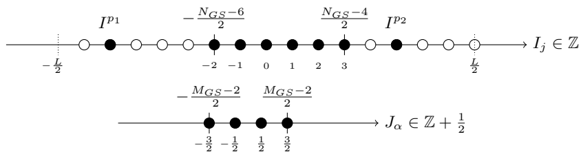
Figure 8: Integer configuration for the particle-particle excitation, explicit numbers for L = 16 , N_{GS} = 10 , M_{GS} = 5 .
