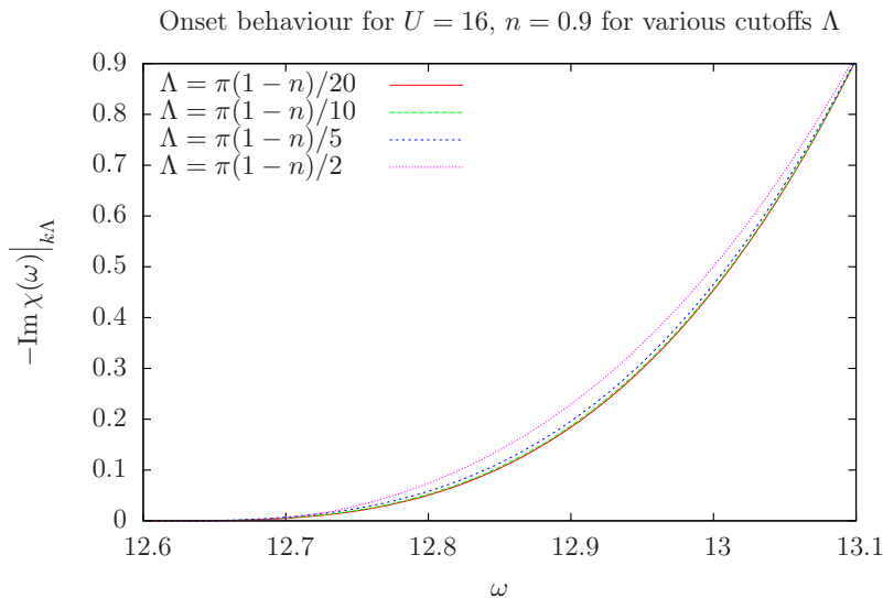
Figure 14: Example of the form of (103) for U = 16 , n = 0.9 for various values of the cutoff \Lambda , normalised such that
