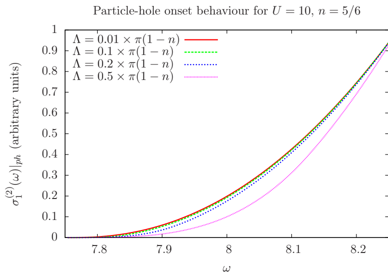
Figure 16: Contribution to onset of \sigma_1^{(2)}(\omega) from particle-hole excitation in (121) for U = 10, n = 5/6
