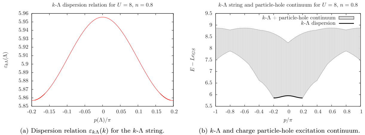
Figure 5: k - \Lambda string dispersion and particle-hole excitation continuum above this for U = 8 , n = 0.8 . For small momenta, the k - \Lambda string dispersion marks the lower edge of a continuum described by additional excitations e.g. particle-hole excitations in the charge sector.
