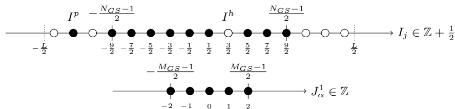
Figure 2: Configuration of the integers for the particle-hole excitation above the ground state, explicit numbers given are for L = 16 , N_{GS} = 10 , M_{GS} = 5
