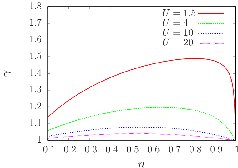
Figure 15: Value of exponent \gamma for various U and n
