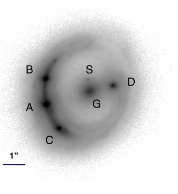
Figure 1. Keck AO image ( K' band) of the gravitational lens RXJ1131-1231. The lensed AGN image of the spiral source galaxy are marked by A, B, C and D, and the star-forming regions in the background spiral galaxy form plentiful lensed features. The foreground main lens and the satellite are indicated by G and S, respectively.
