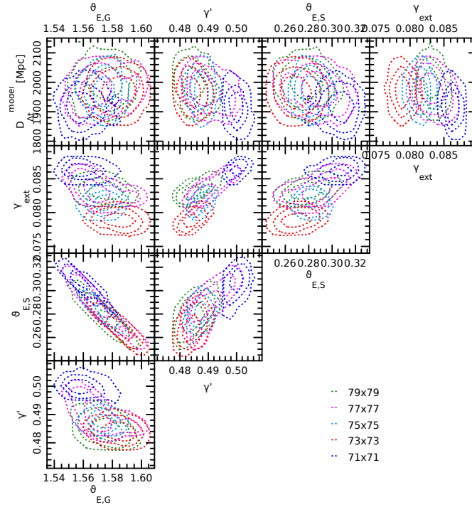
Figure 11. Posterior of the key lens model parameters for RXJ1131–1231 and the time delays. We use the PSF size, 59 \times 59 , for convolution of the spatially extended lens and arcs. We show the constraints from Markov chains of different source resolutions: 71 \times 71 , 73 \times 73 , 75 \times 75 , 77 \times 77 , and 79 \times 79 . The contours mark the 68.3%, 95.4%, and 99.7% credible regions for each source resolution. The spread in the constraints from different chains allow us to quantify the systematic uncertainty due to the pixelated source resolution.
