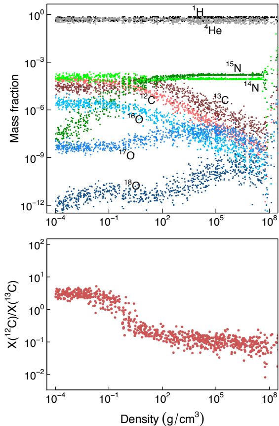
Fig. 8.— Simulated final abundances of ^1\text{H} , ^4\text{He} , ^{12}\text{C} , ^{13}\text{C} , ^{14}\text{N} , ^{15}\text{N} , ^{16}\text{O} , ^{17}\text{O} , and ^{18}\text{O} (top panel) and carbon isotopic mass fraction ratio (bottom panel) in processed matter versus stellar density. The results are obtained from the same Monte Carlo simulation shown in Figure 5 (blue circles) and include the random sampling of nuclear reaction rates and initial composition.
