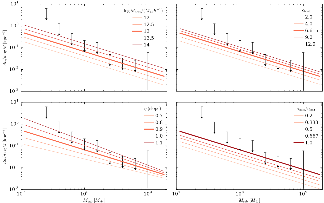
Figure 13. Comparison between the 95% confidence limits (black squares) on the projected density of substructures, dn/d\log M , and the predictions (lines) for various properties of the host halo and its substructure distribution. The thick line in each panel assumes M_{\text{host}} = 10^{13} M_{\odot} h^{-1} , a median halo concentration for that mass ( c_{\text{host}} = 6.615 ), a typical log–log slope ( \eta = 0.9 ) for the subhalo mass function, and that the radial distribution of subhalos matches that of dark matter ( c_{\text{subs}}/c_{\text{host}} = 1 ). Each panel varies only one of the four assumptions listed above. The varying assumption is showed on the upper right corner of each panel.
