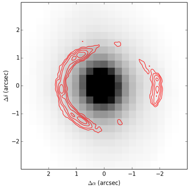
Figure 4. The SDP.81 system. Grayscale shows HST/WFC3 F160W data, while red contours show ALMA continuum emission in band 6.
