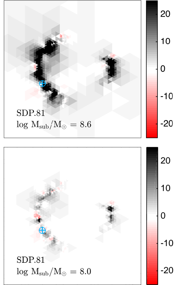
Figure 9. Search for additional substructure. Top panel shows a map of linearized \Delta\mathcal{E} for a second subhalo, of mass M = 10^{8.6}M_\odot , following the inclusion of one subhalo of mass M \approx 10^9M_\odot at the location of the blue circled cross, using a joint analysis of bands 6 and 7. After adding the subhalo to the main lens model, no additional subhalos of this mass are found. The bottom panel shows a similar analysis for a lower mass subhalo, showing a marginal improvement of \mathcal{E} at another point near the first detection.
