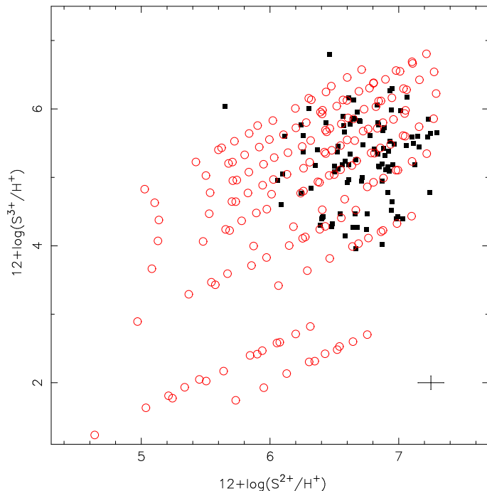
Figure 3. Such as Fig. 2 but for the Ionic abundances S^{3+}/H^+ vs. S^{2+}/H^+ computed using the IR-sample (Table 6) and the IR-lines method (see Sect. 4.2).
