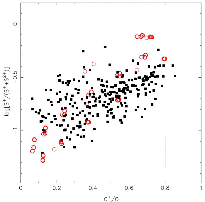
Figure 2. Ionic abundances S + /(S + + S 2+ ) vs. O + /O. Black squares represent observational ionic determinations computed using the data from Table 5 and the Visible-lines method (see Sect. 4.2). Open circles represent ionic abundances predicted by our models (see Sect. 3). The error bar represents typical uncertainties as defined in Sect 4.1.
