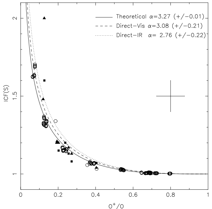
Figure 4. Ionization Correction Factor for the sulphur vs. O^+/O . Squares and triangles represent direct estimations (see Table 7) of the ICF taking into account the S^{2+} ionic abundance values estimated from the Visible-sample (Direct-Vis) and the IR-sample (Direct-IR), respectively. Circles represent estimations of our models. Curves represent the fittings to the Eq. 2: Solid line shows the best fit obtained using our models and dashed and dotted lines the ones obtained using the observational estimations, as indicated. The \alpha values of the best fits are indicated in the legend. The error bars represent typical uncertainties as defined in Sect 4.2.
