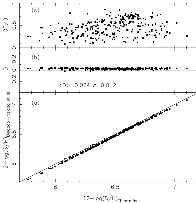
Figure 7. Idem Fig. 5 for the ICF proposed by Delgado-Inglada et al. (2014)
