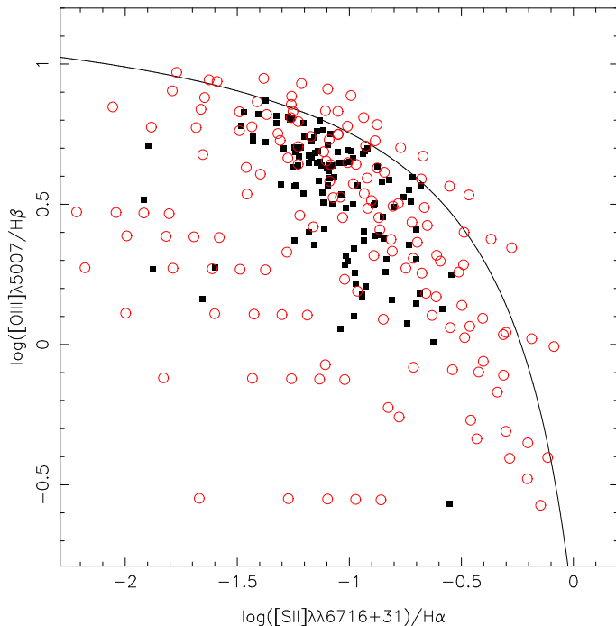
Figure 1. \log([\text{O III}]\lambda 5007/\text{H}\beta) vs. \log([\text{S II}]\lambda\lambda 6716+31/\text{H}\alpha) diagnostic diagram. Solid line, taken from Kewley et al. (2001), separates objects ionized by massive stars from those containing active nuclei and/or shock-excited gas. Black squares represent the objects in our sample. Open circles represent estimations predicted by our models (see Sect. 3).
